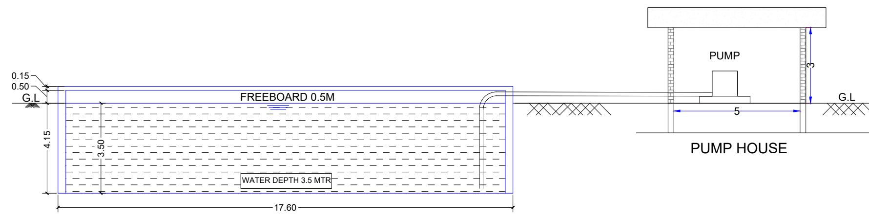
UNDER GROUND RESERVOIR ELEVATION
