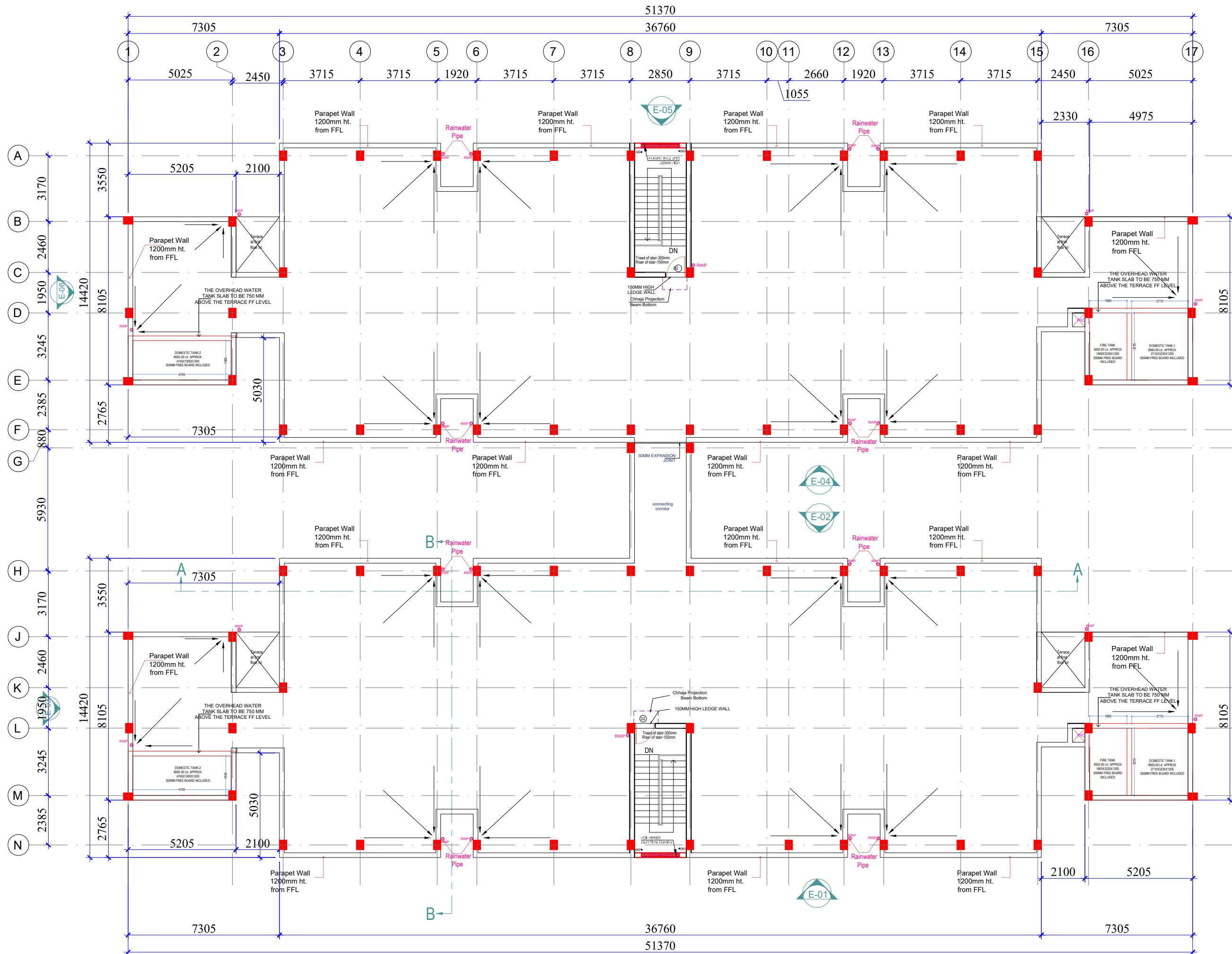
TERRACE FLOOR PLAN +6600 mm Page 279 of 414
