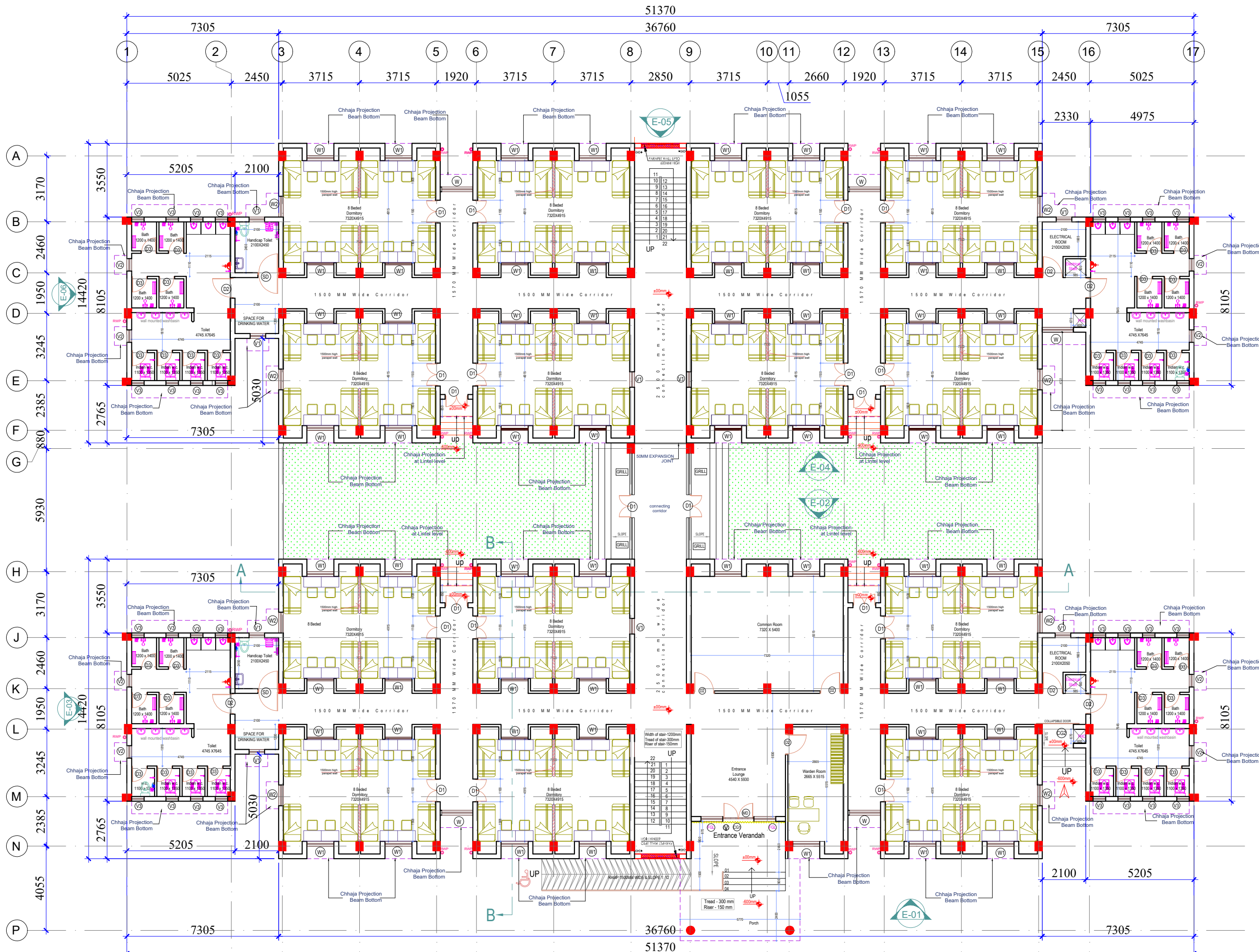
GROUND FLOOR PLAN ±00mm Page 270 of 414
