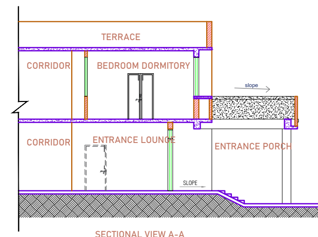
SECTIONAL VIEW A-A
