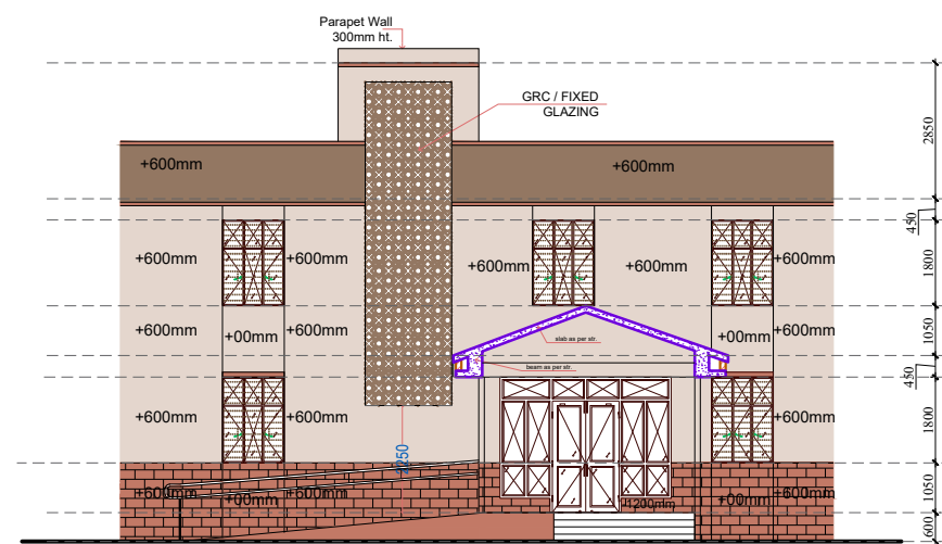
SECTIONAL FRONT VIEW
