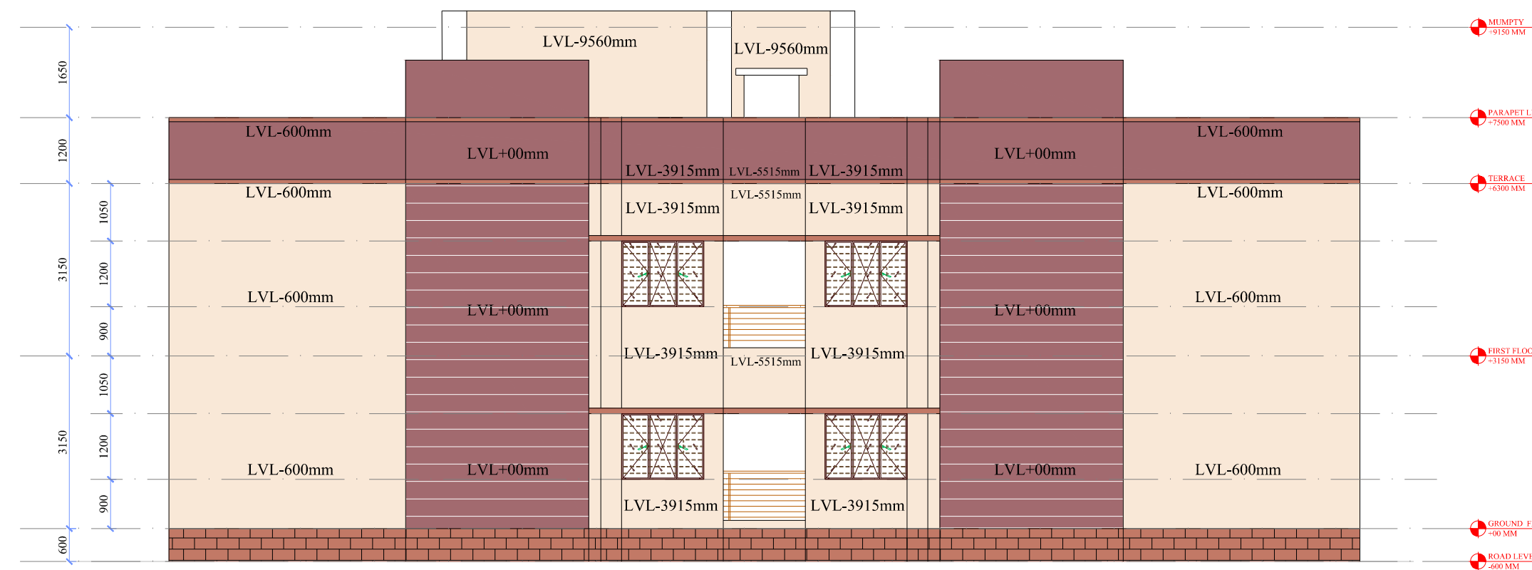
SIDE ELVATION
