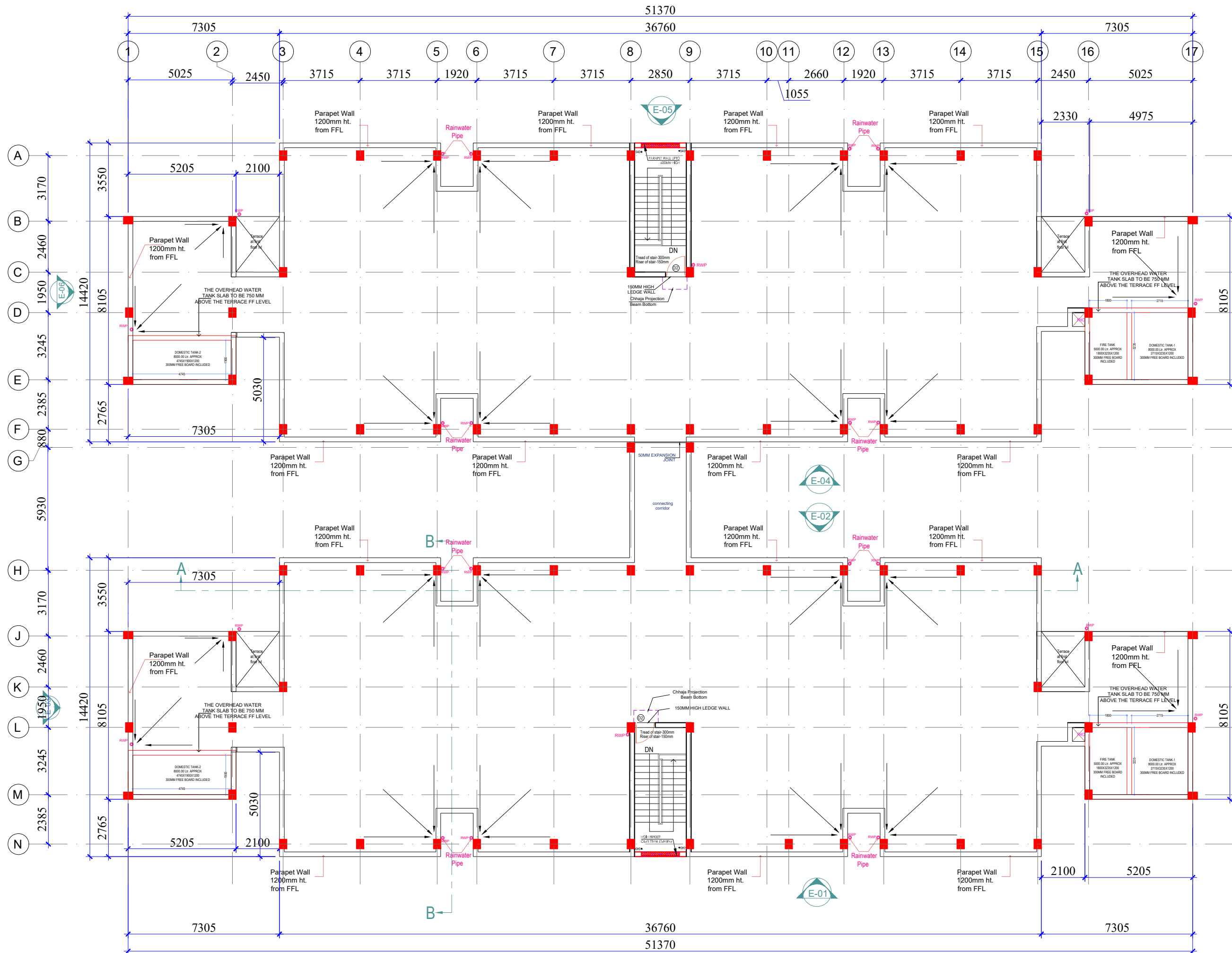
TERRACE FLOOR PLAN +6600 mm Page 272 of 414
