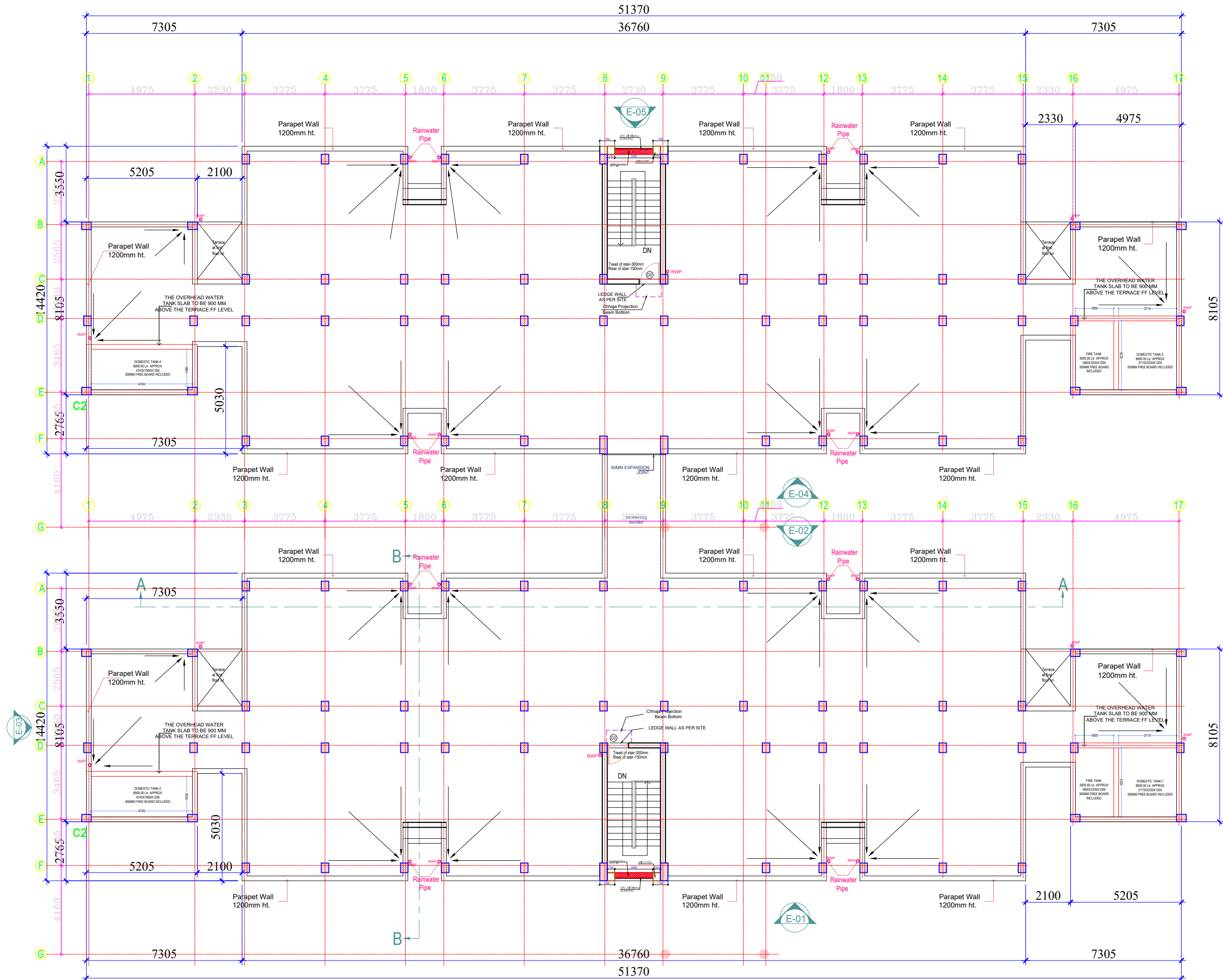
TERRACE FLOOR PLAN +6600 mm Page 282 of 370
