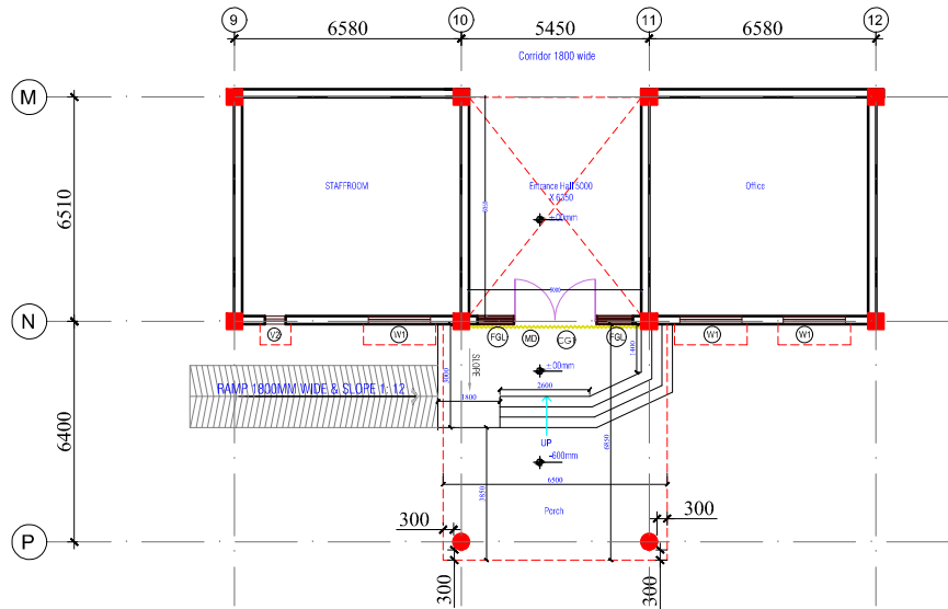
GROUND FLOOR PLAN ENTRANCE PORCH
