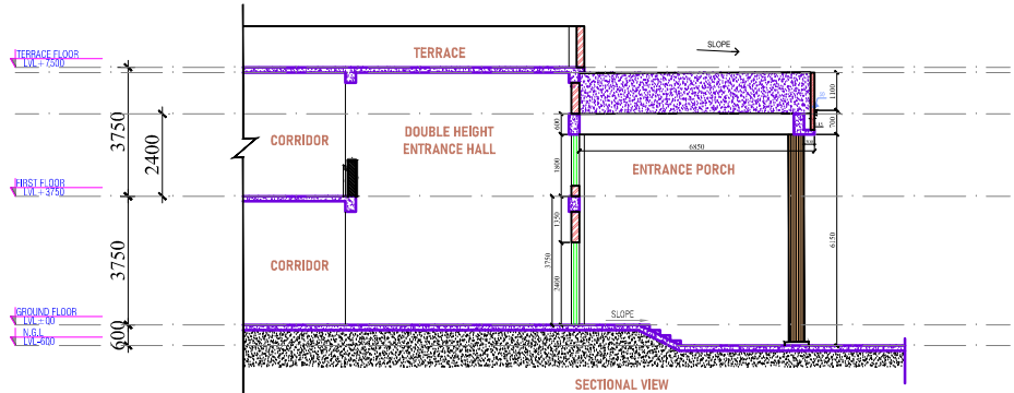
SECTIONAL VIEW ENTRANCE PORCH
