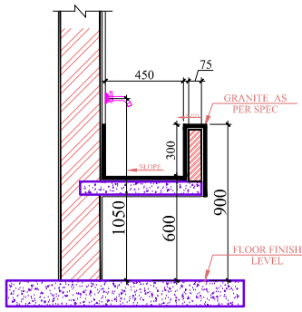
TROUGH TYPICAL SECTION
