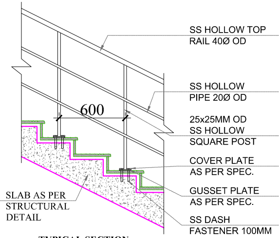
TYPICAL SECTION STAIRCASE RAILING
