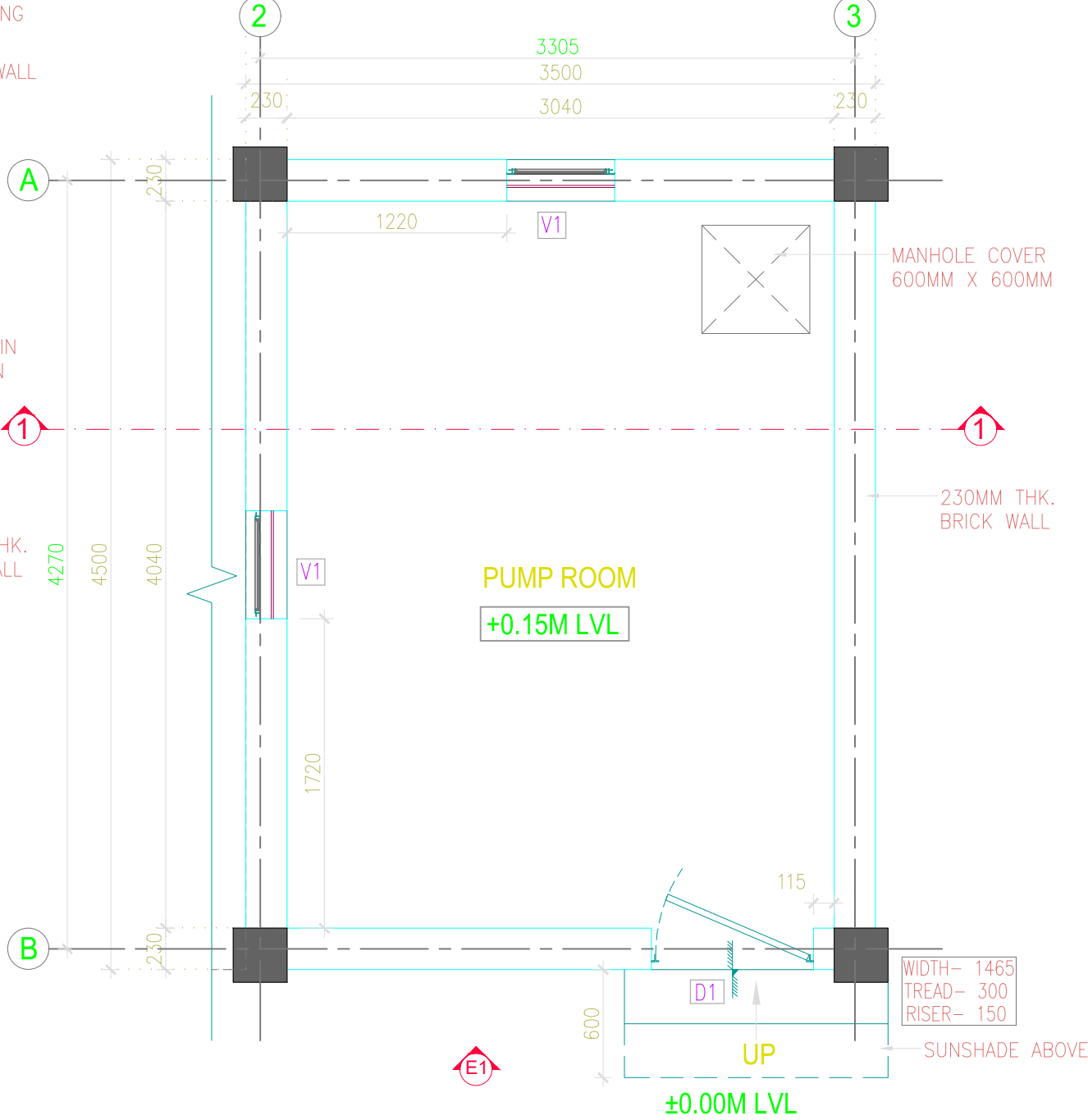
PUMP ROOM PLAN
