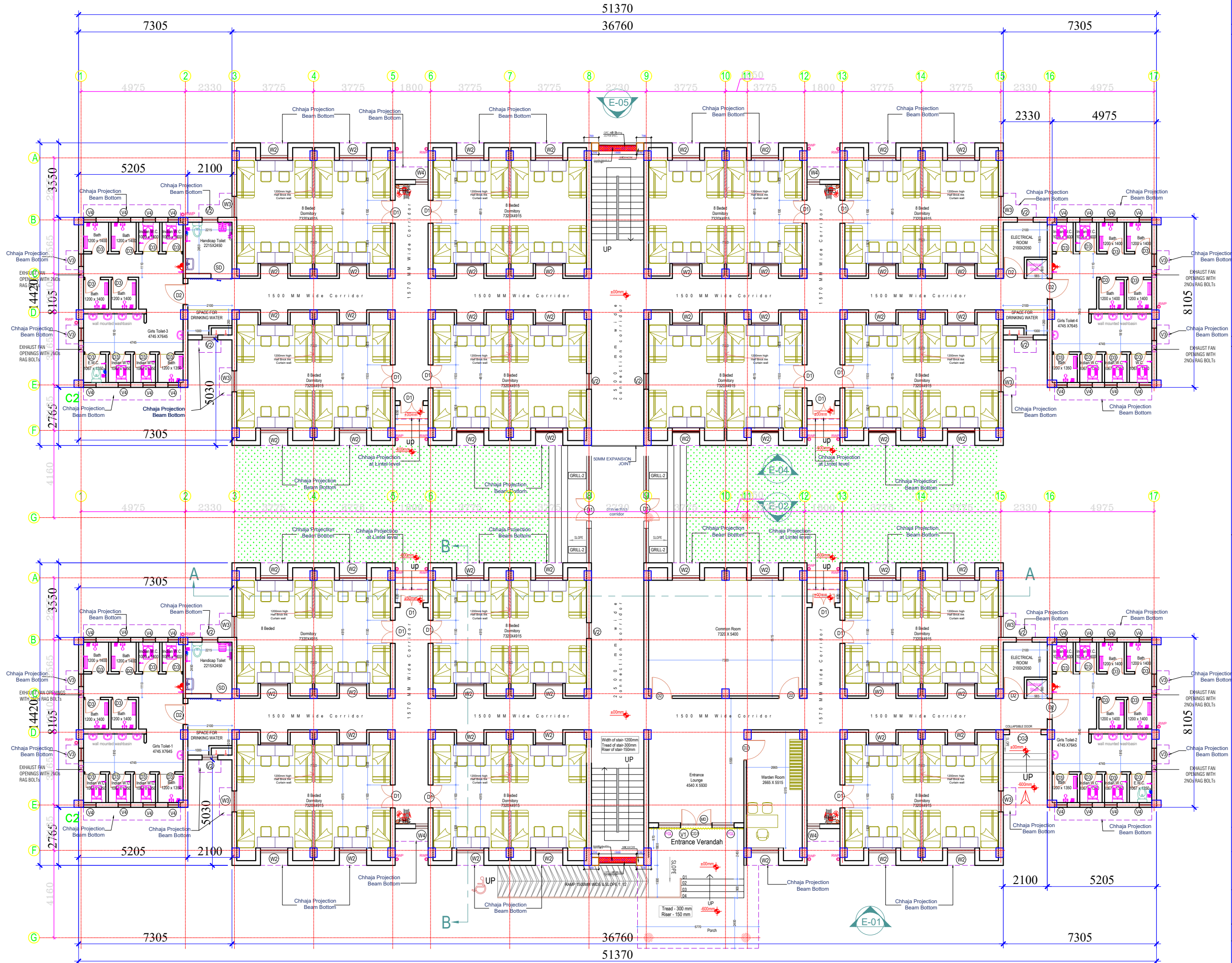
GROUND FLOOR PLAN \pm 00 mm Page 280 of 370
