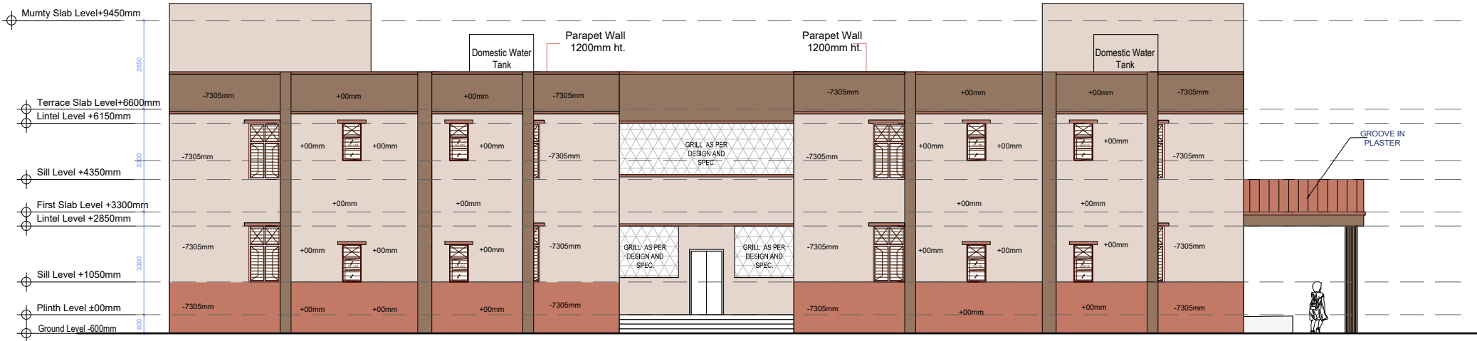
SIDE ELEVATION E-03
