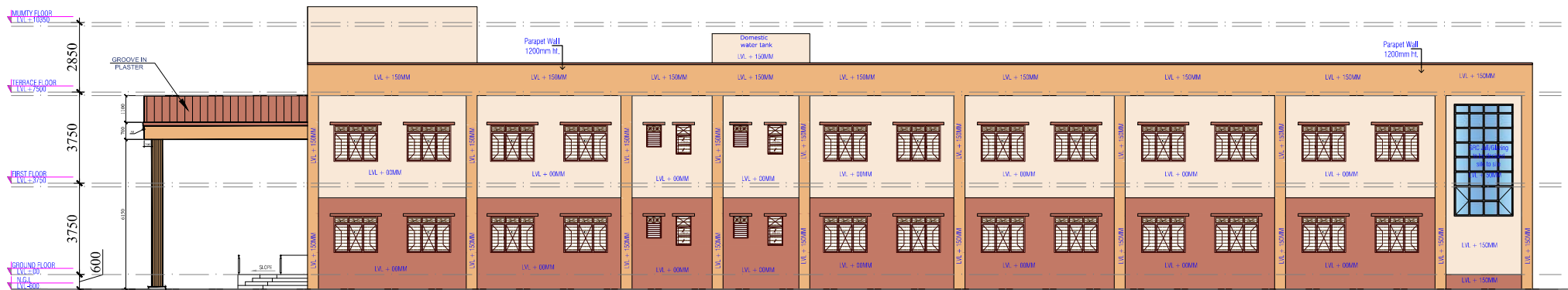
RIGHT SIDE ELEVATIONS
