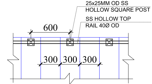
PLAN STAIRCASE RAILING
