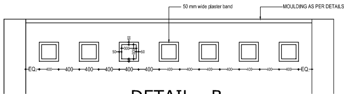
DETAIL - B
