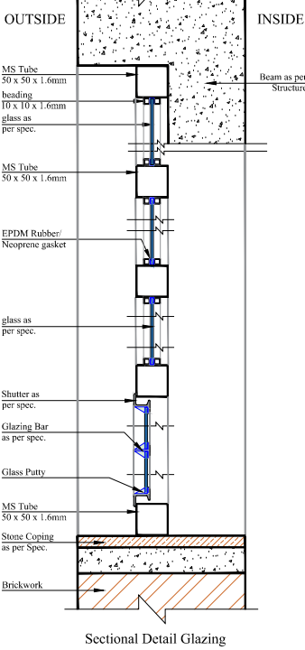
Sectional Detail Glazing
