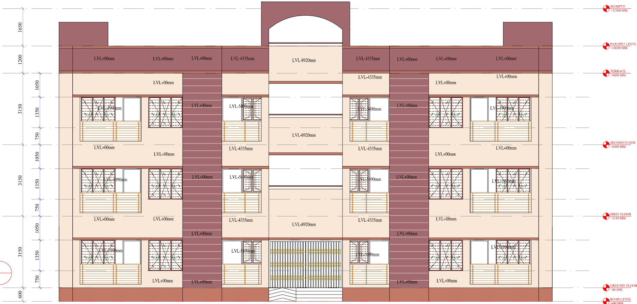
FRONT ELVATION
