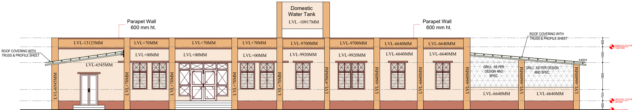
BOYS ENTRY SIDE ELEVATION
