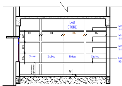
LAB STORE- RCC SHELVES DETAIL
