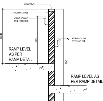
RAMP RAILING DETAIL
