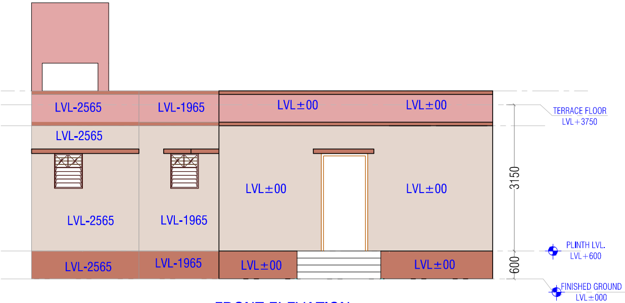
FRONT ELEVATION
