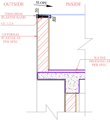
TERRACE PARAPET WALL TYPICAL COPING DETAIL
