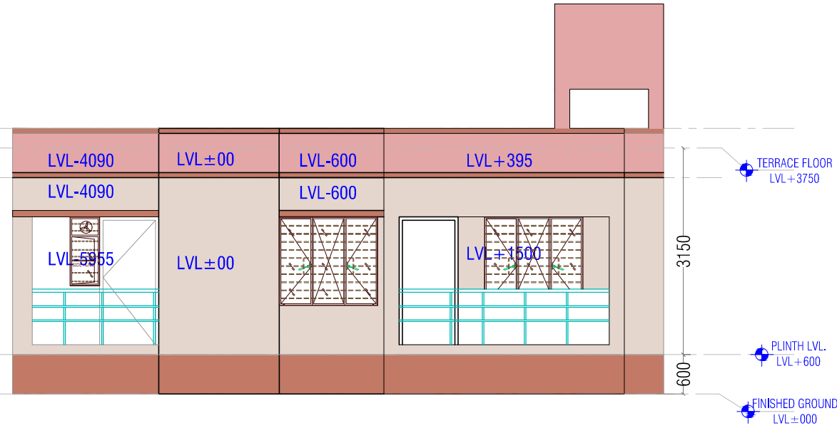
BACKSIDE ELEVATION
