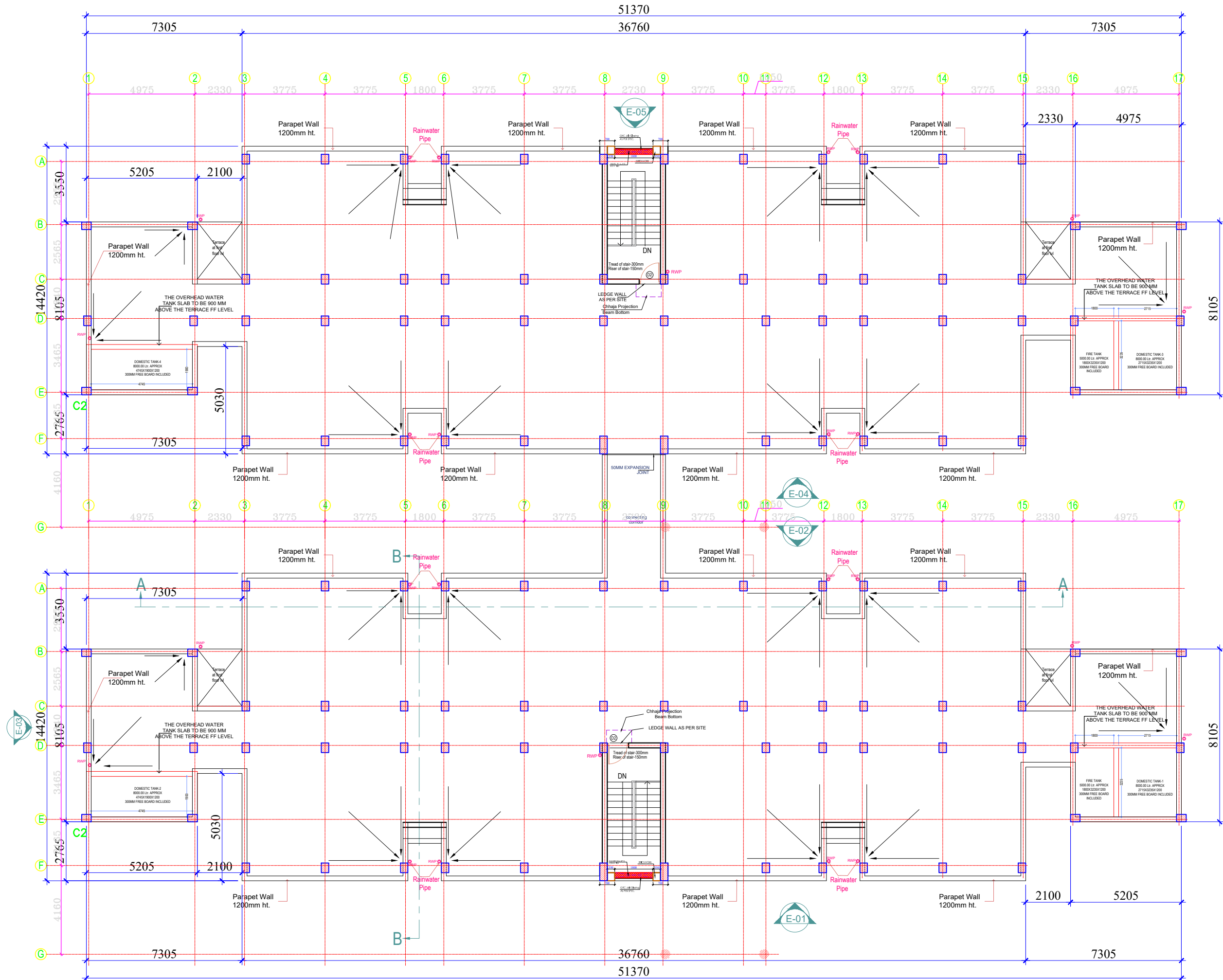
TERRACE FLOOR PLAN +6600 mm Page 276 of 370
