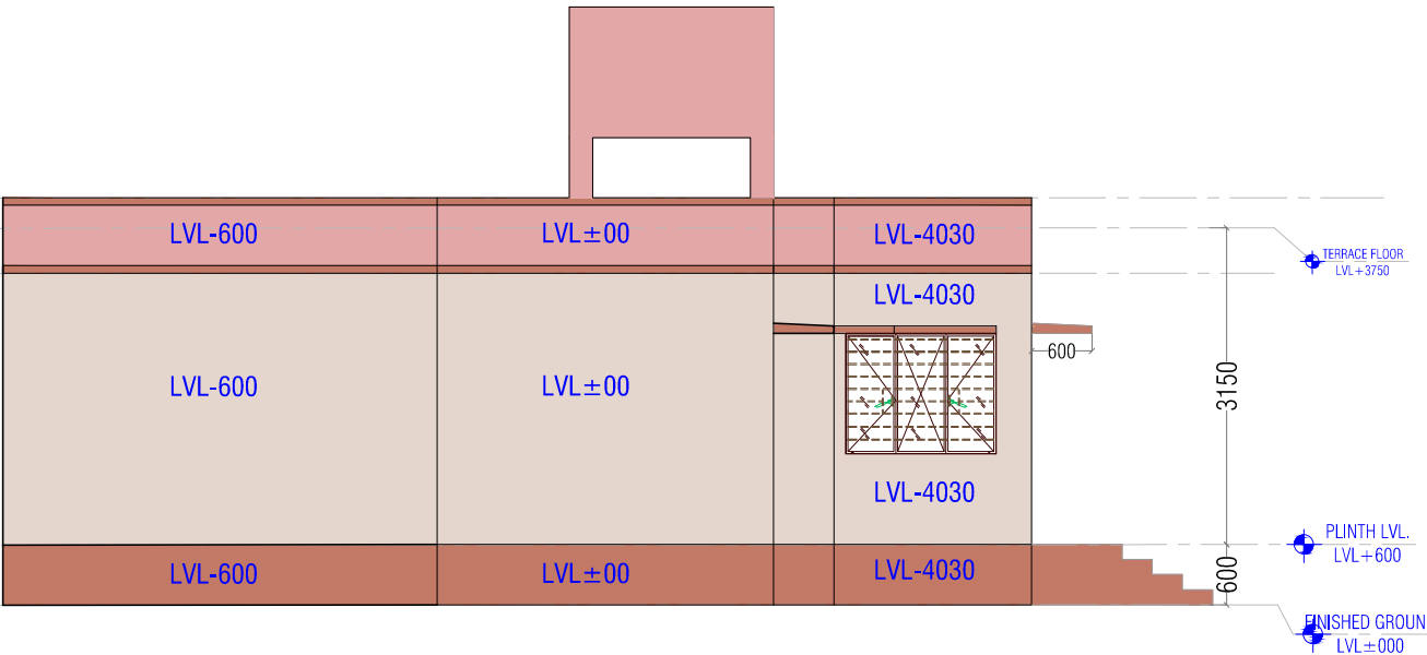
BEDROOM SIDE ELEVATION
