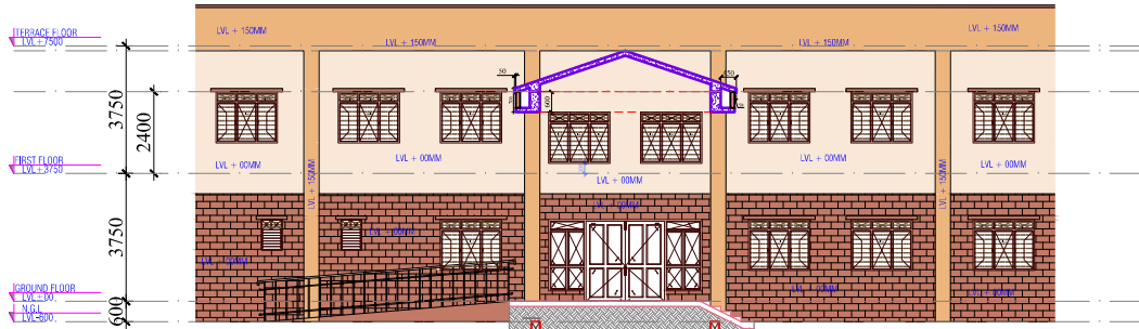
SECTIONAL FRONT VIEW ENTRANCE PORCH
