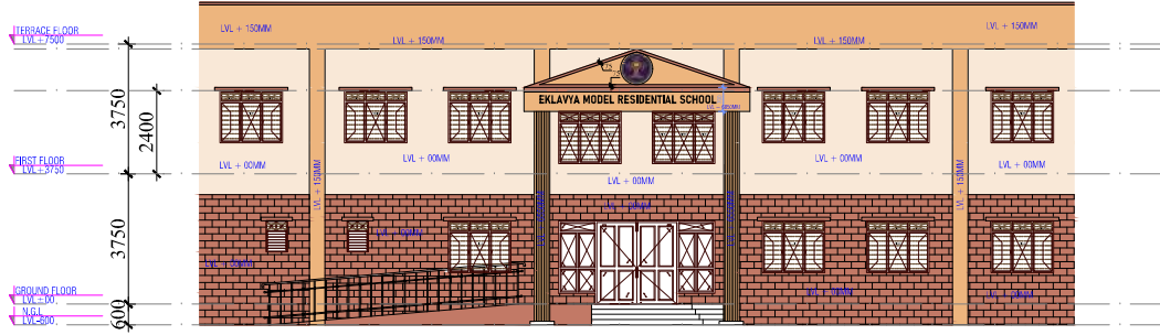
FRONT ELEVATION ENTRANCE PORCH
