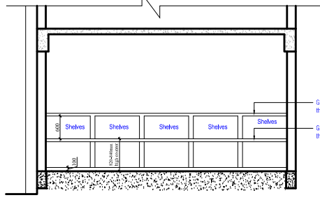
LAB RCC 820-840MM HIGH COUNTER WITH SHELF ABOVE- RCC SHELVES DETAIL
