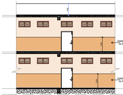
TYPICAL CORRIDOR SECTION
