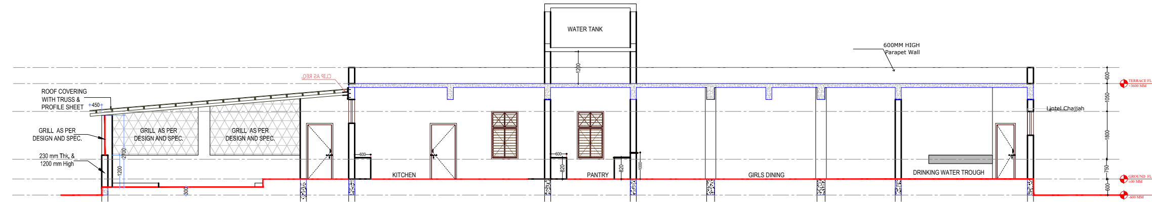
SECTION - BB
