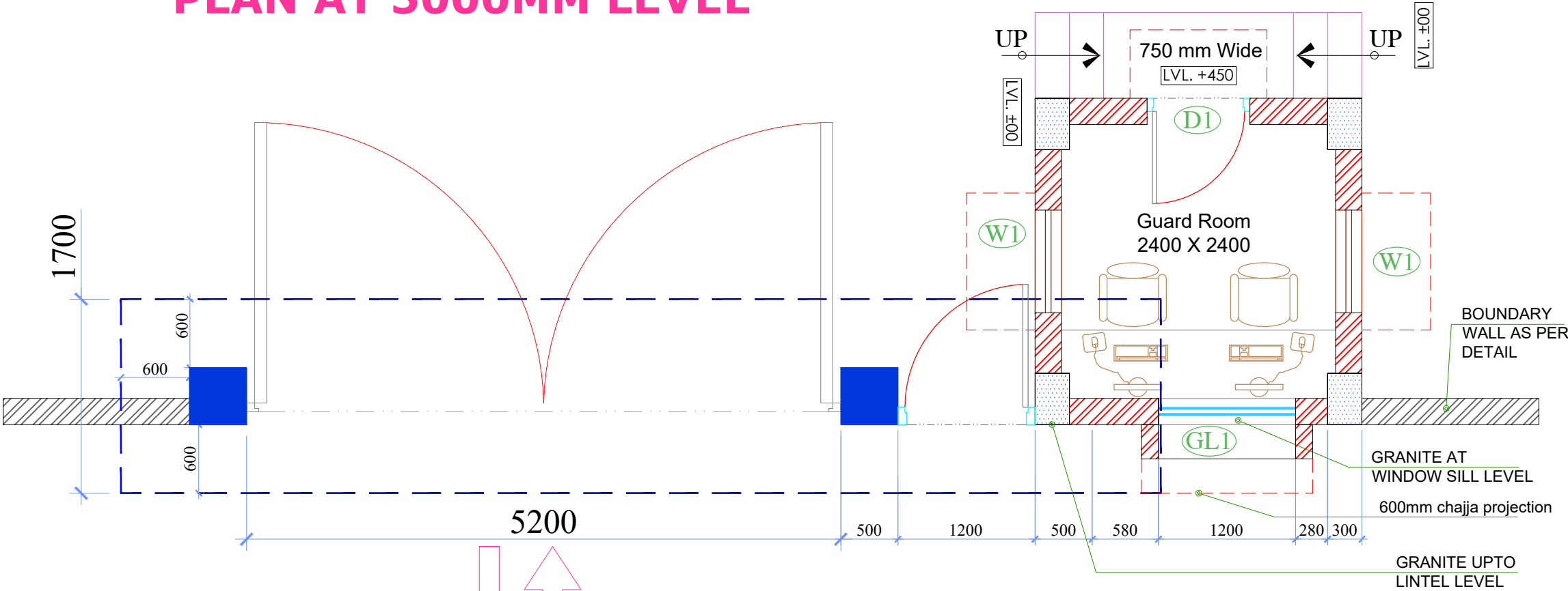
PLAN AT 5000MM LEVEL
