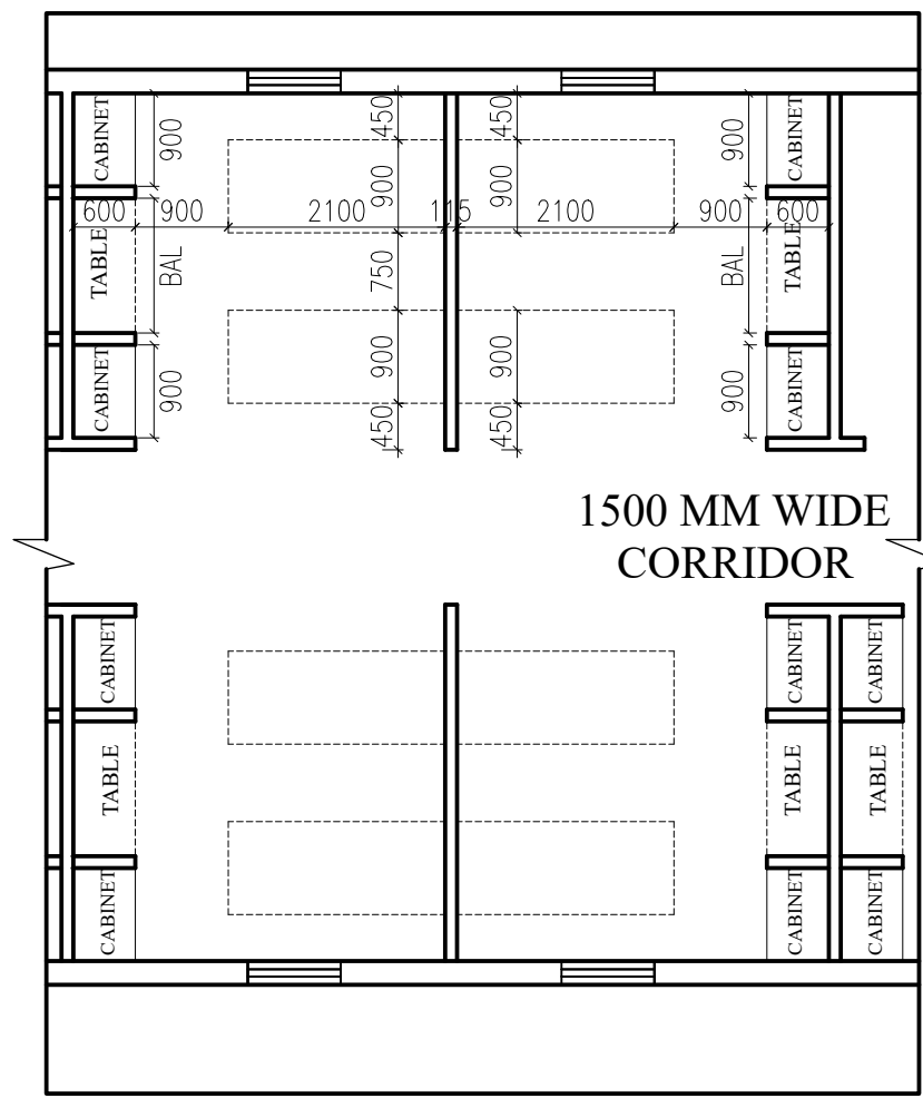
TYPICAL FURNITURE LAYOUT
