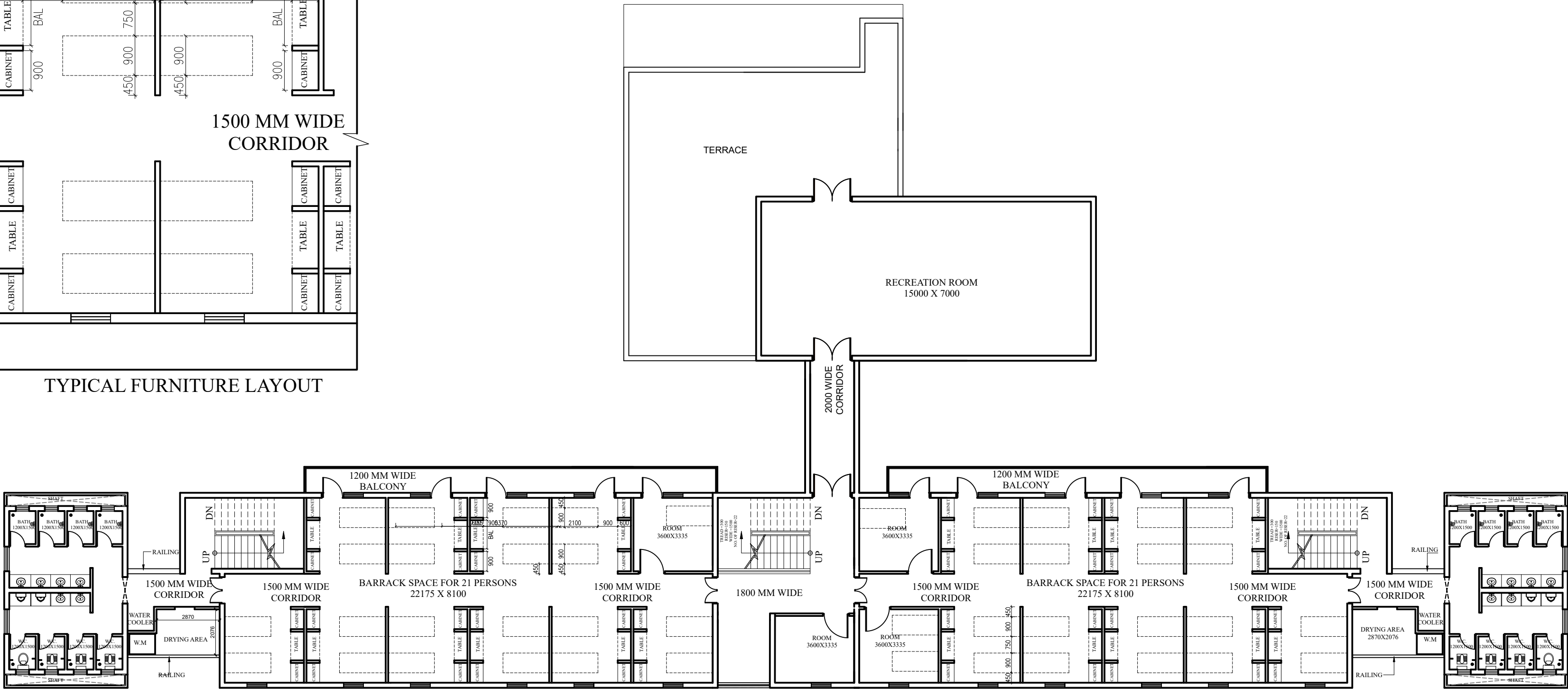
FIRST FLOOR PLAN 761.44 Sqm
