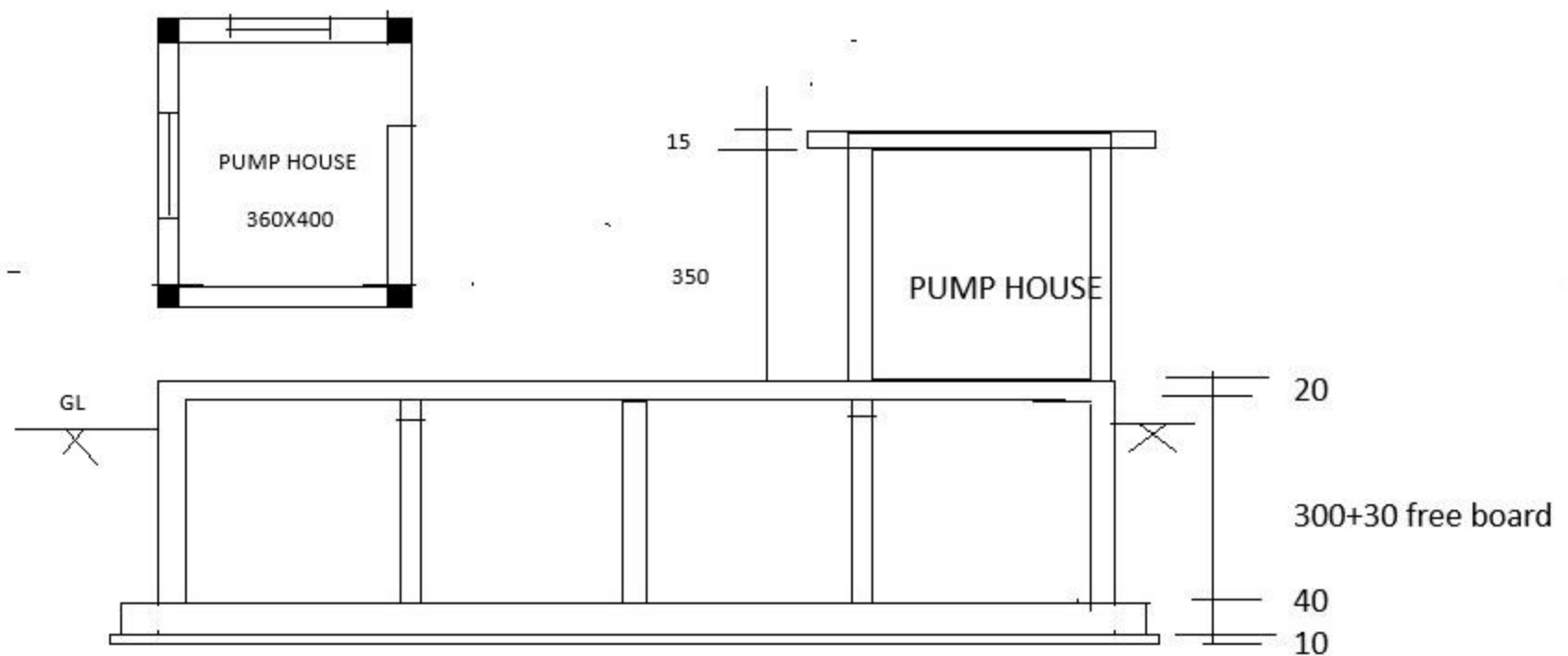
CROSS SECTION
