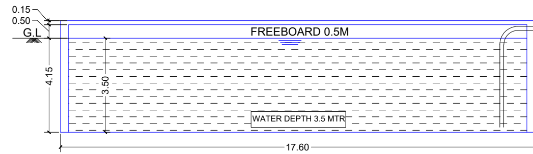
UNDER GROUND RESERVOIR
