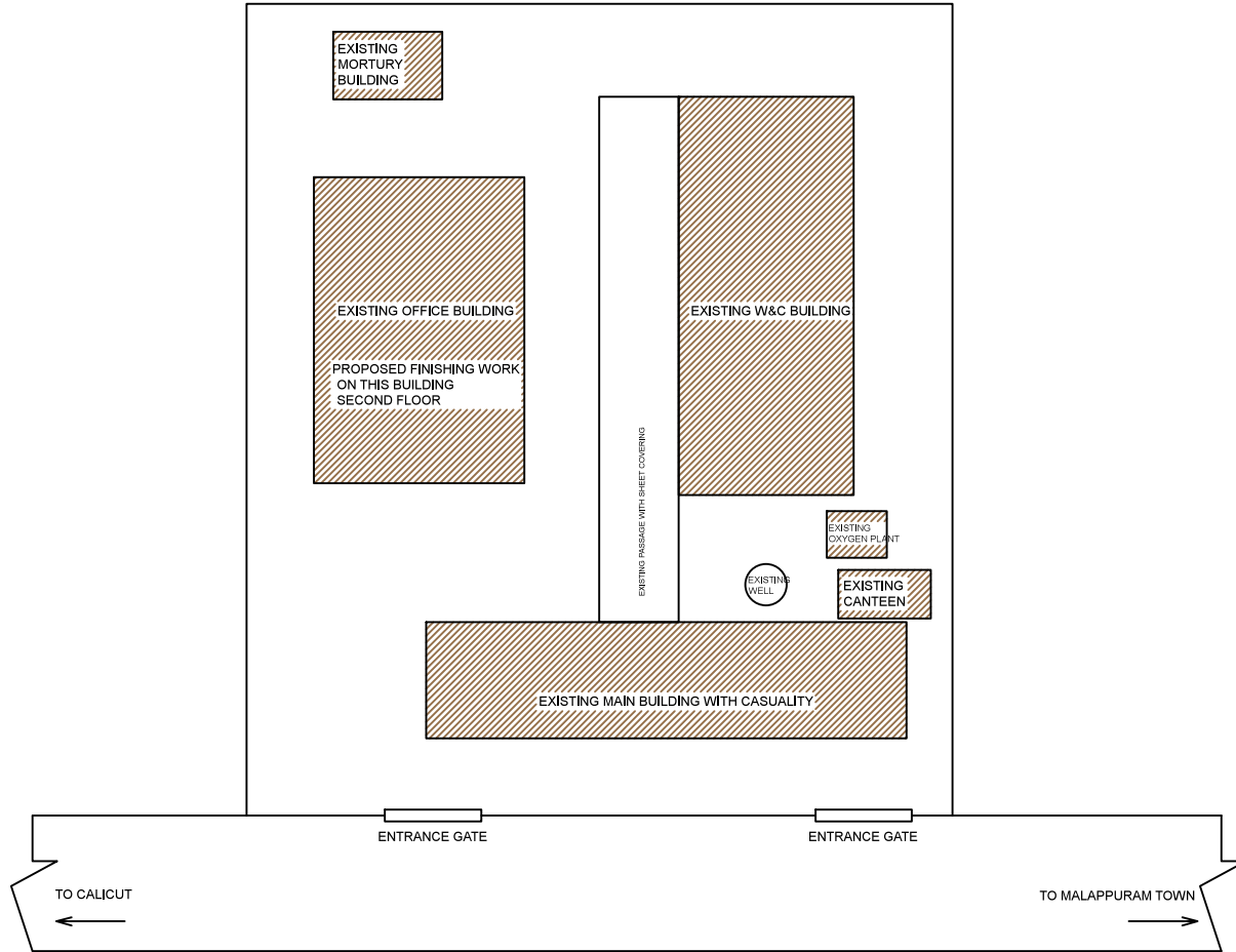
KEY PLAN
