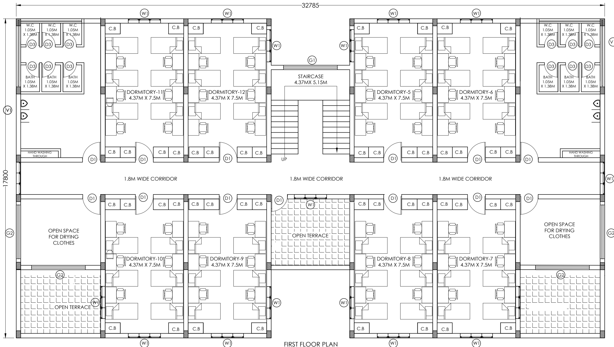
FIRST FLOOR PLAN AREA-502 SQM
