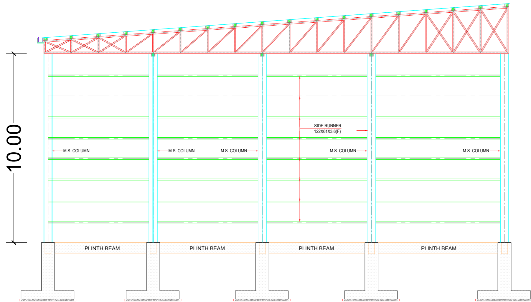
FRONT ELEVATION
