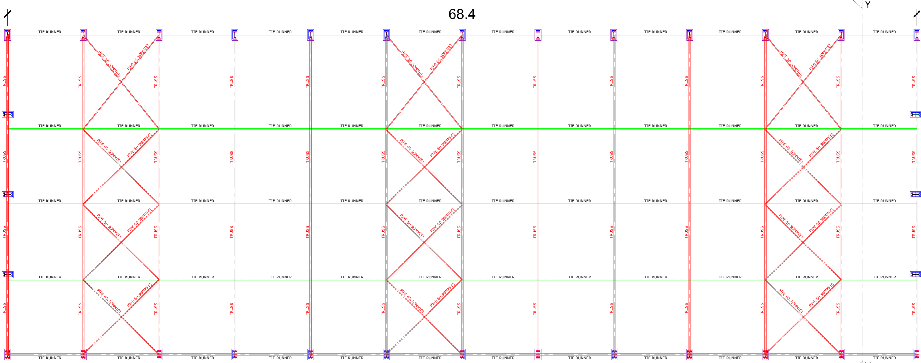
TIE LEVEL PLAN
