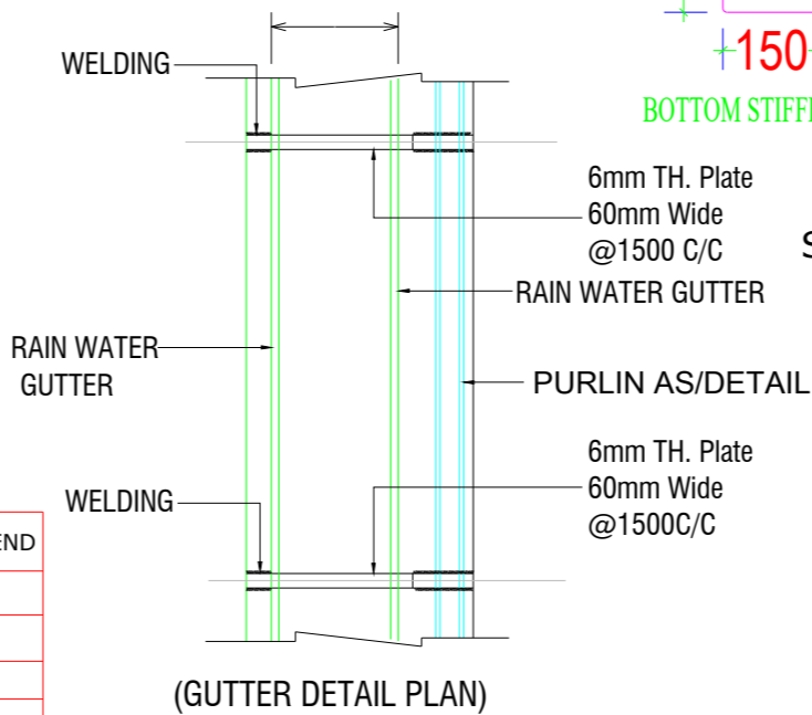
(GUTTER DETAIL PLAN)
