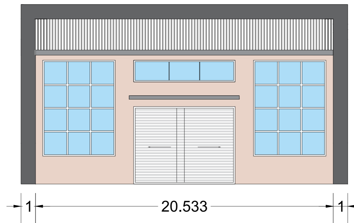
FRONT ELEVATION
