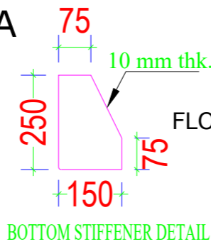
BOTTOM STIFFENER DETAIL
