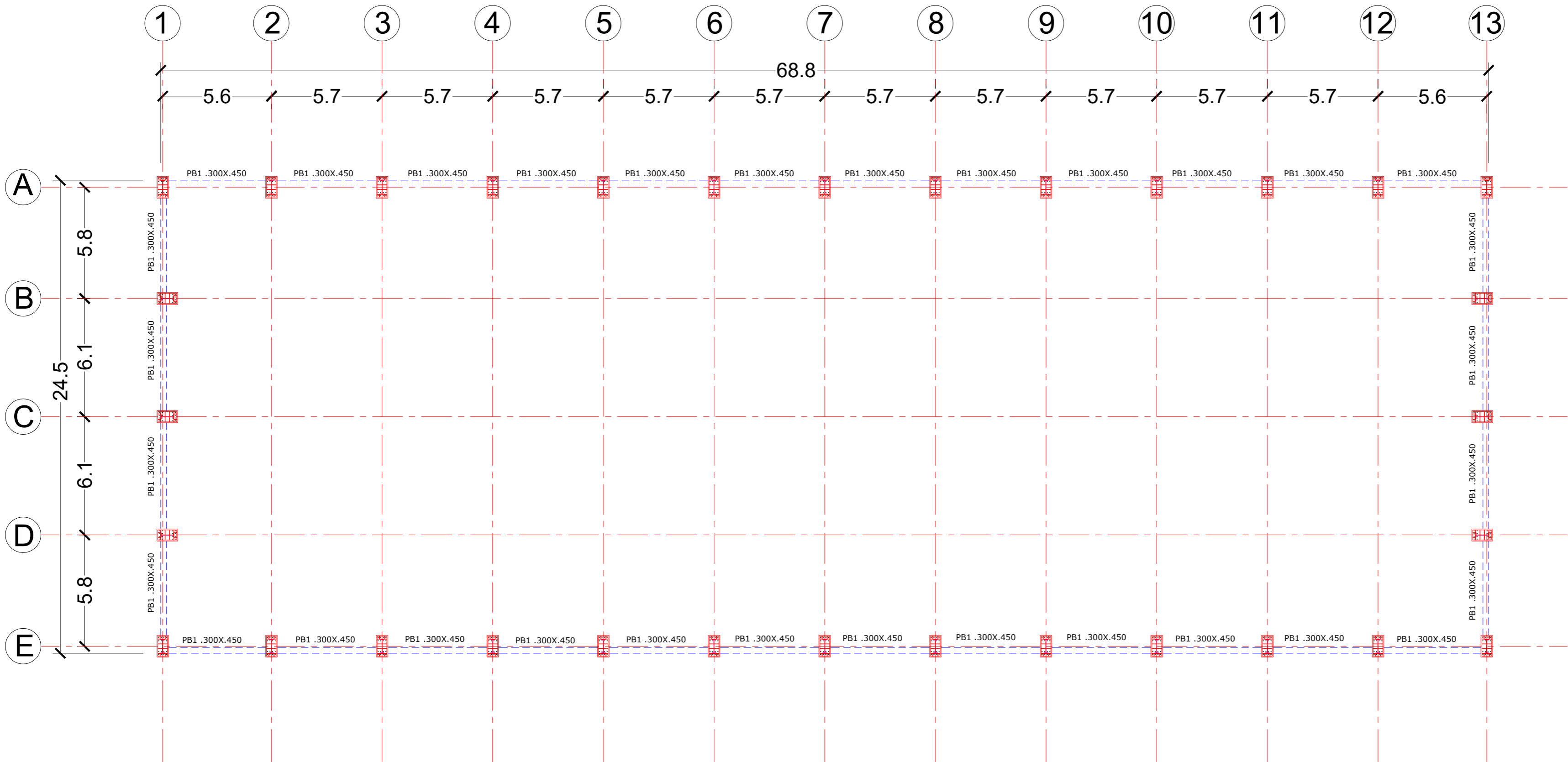
PLINTH BEAM LAYOUT PLAN
