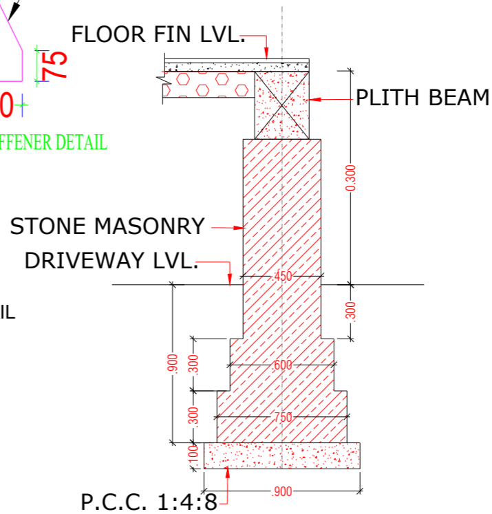
WALL SECTION A-A'
