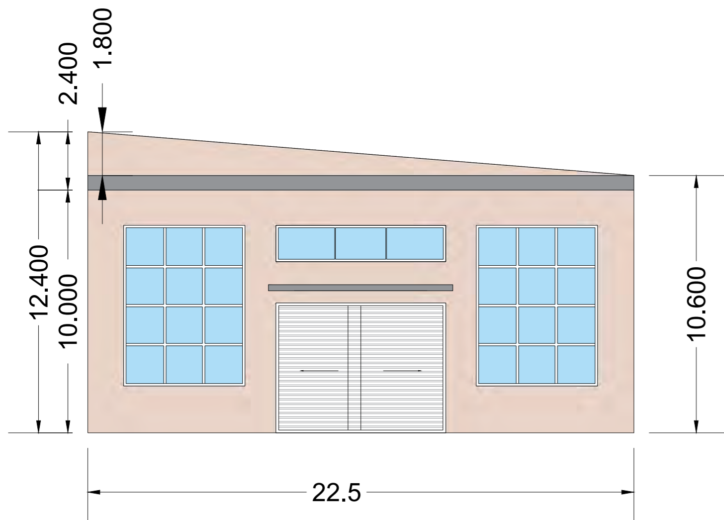
BACK ELEVATION
