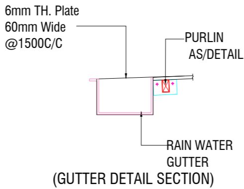
GUTTER DETAIL SECTION
