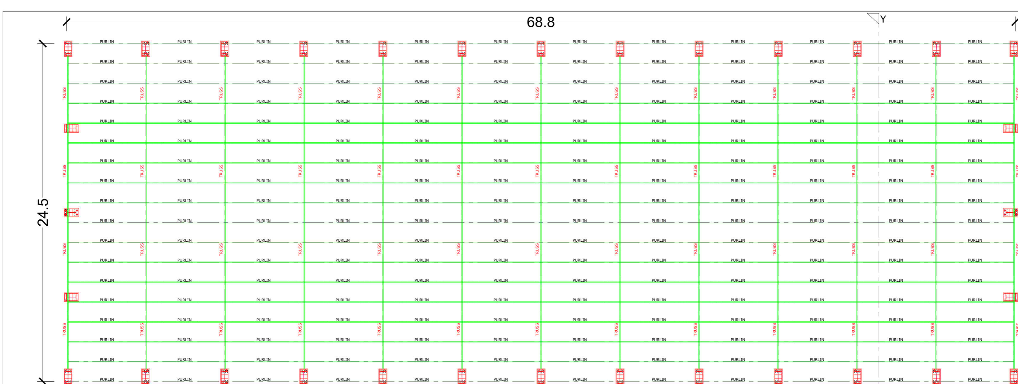
TRUSS PLAN
