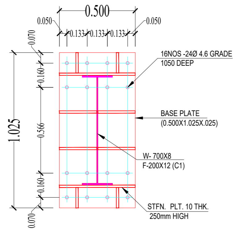
DETAIL OF BASE PLATE-BP1 (0.500X1.025X.025)
