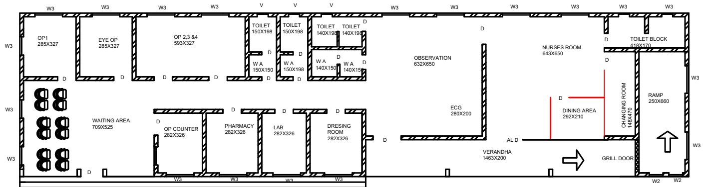
FIRST FLOOR
