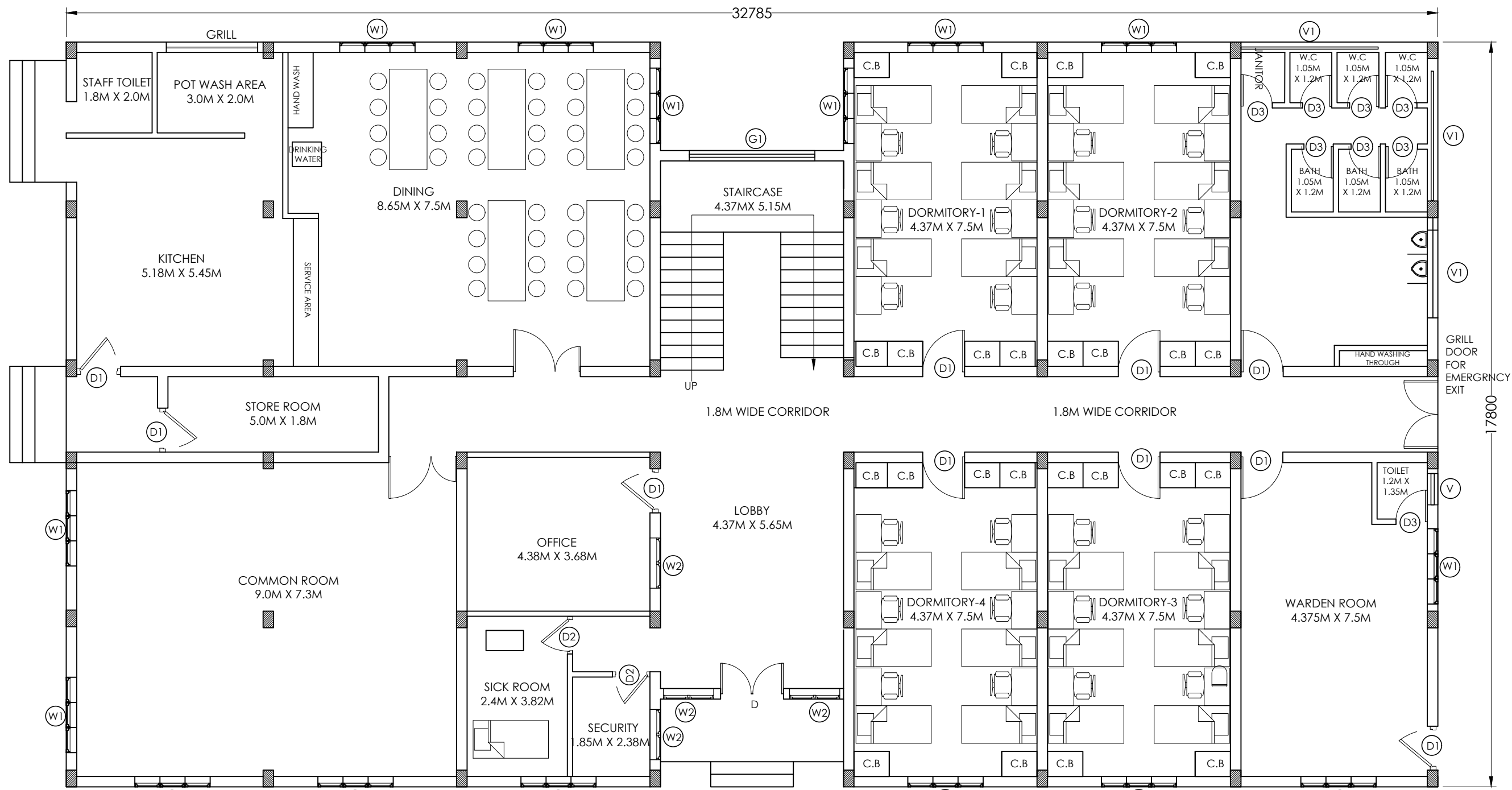
GROUND FLOOR PLAN 563 SQM
