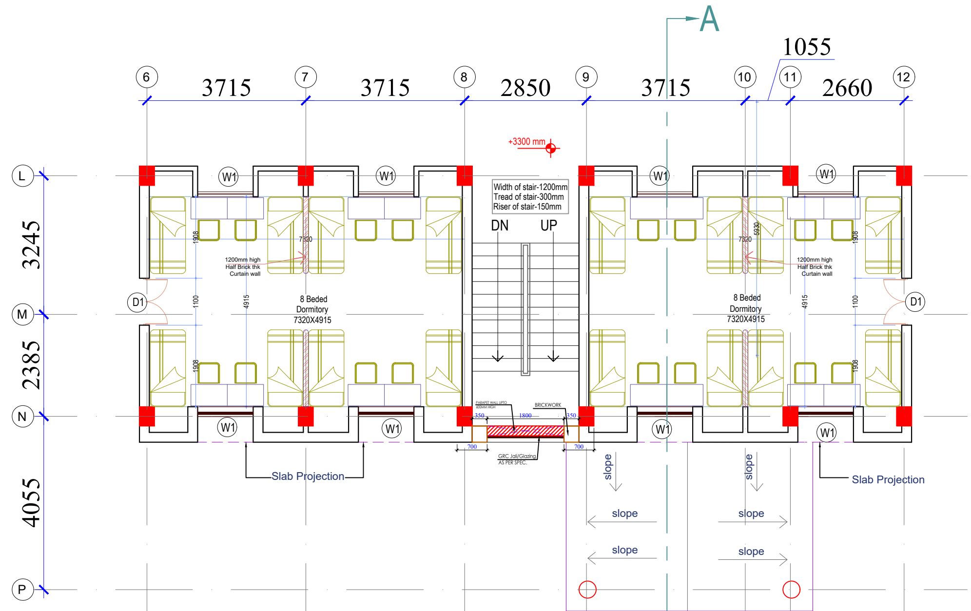
FIRST FLOOR PLAN +3300mm
