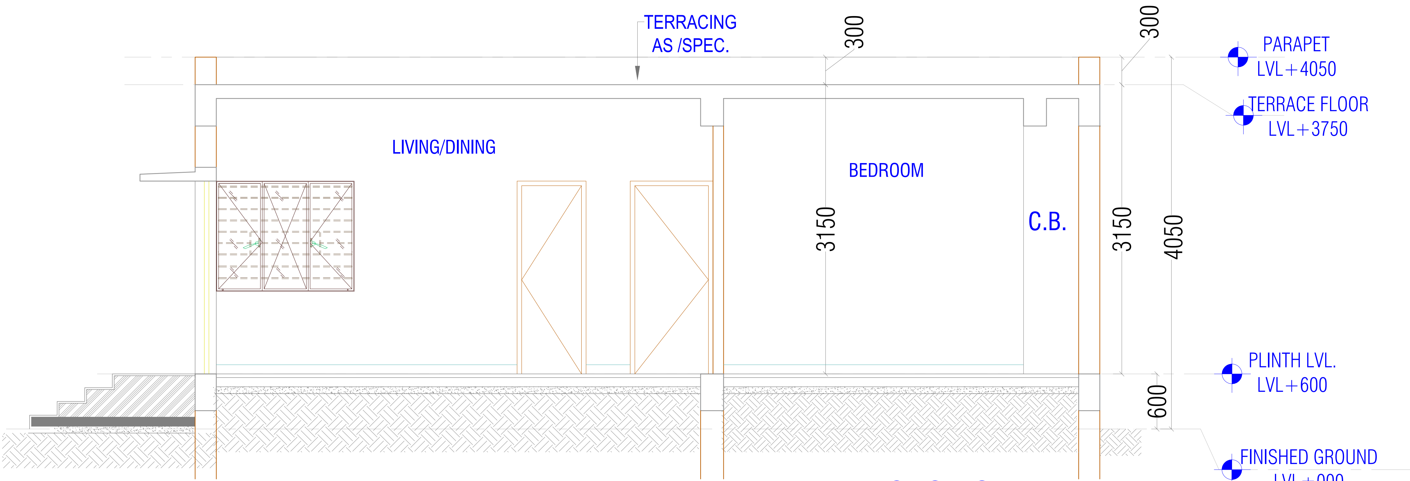
SECTION 2-2'
