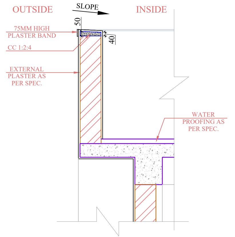
TERRACE PARAPET WALL TYPICAL COPING DETAIL
