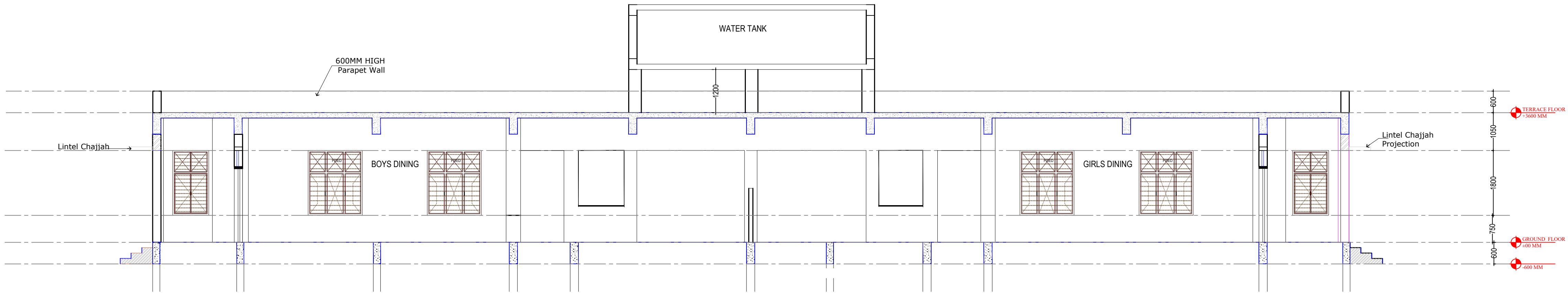
SECTION - AA
