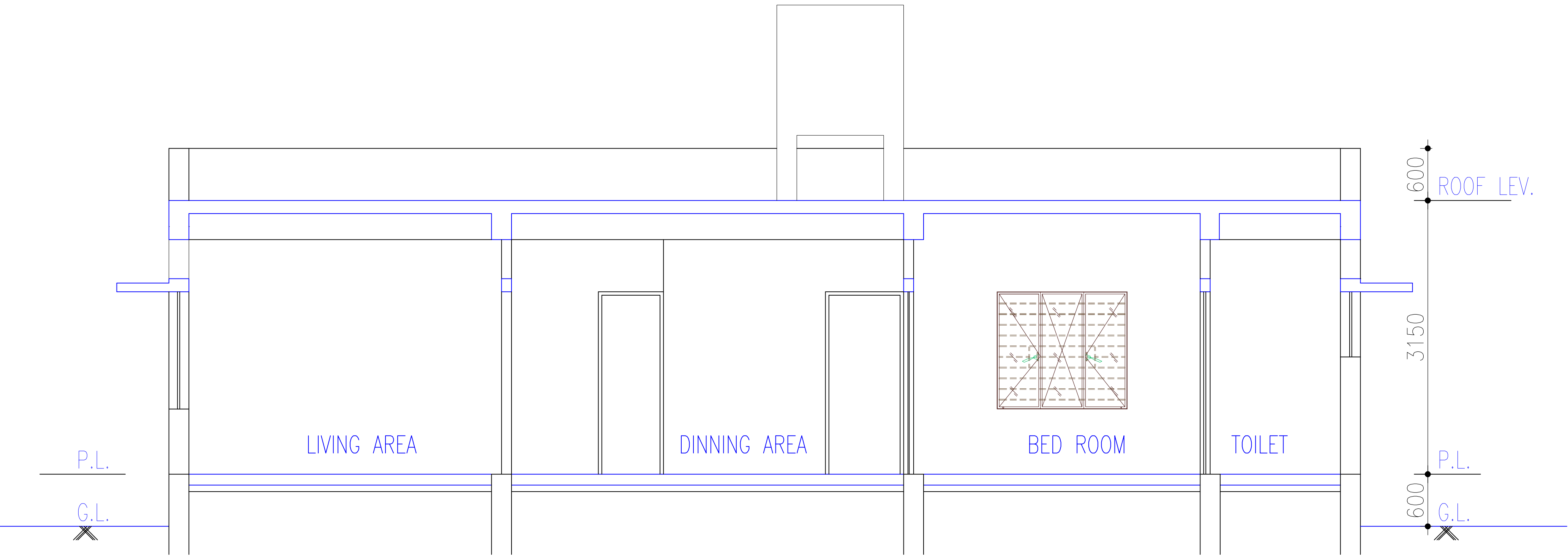
SECTION S1 -
