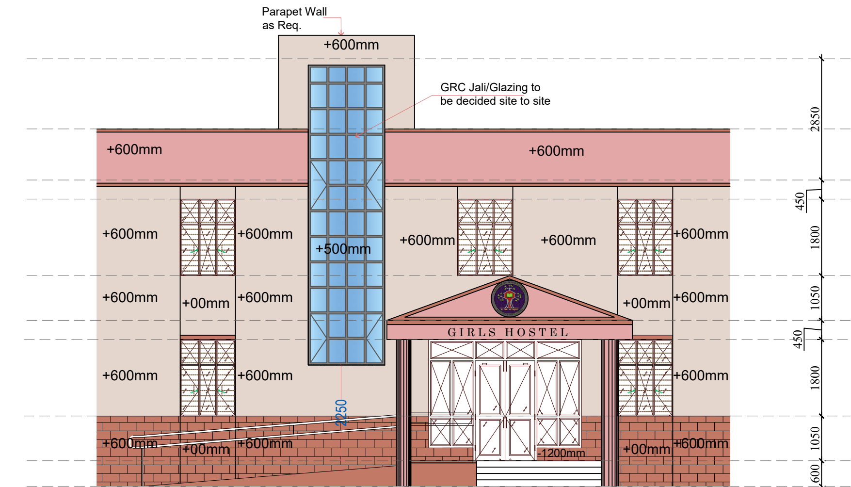
FRONT ELEVATION
