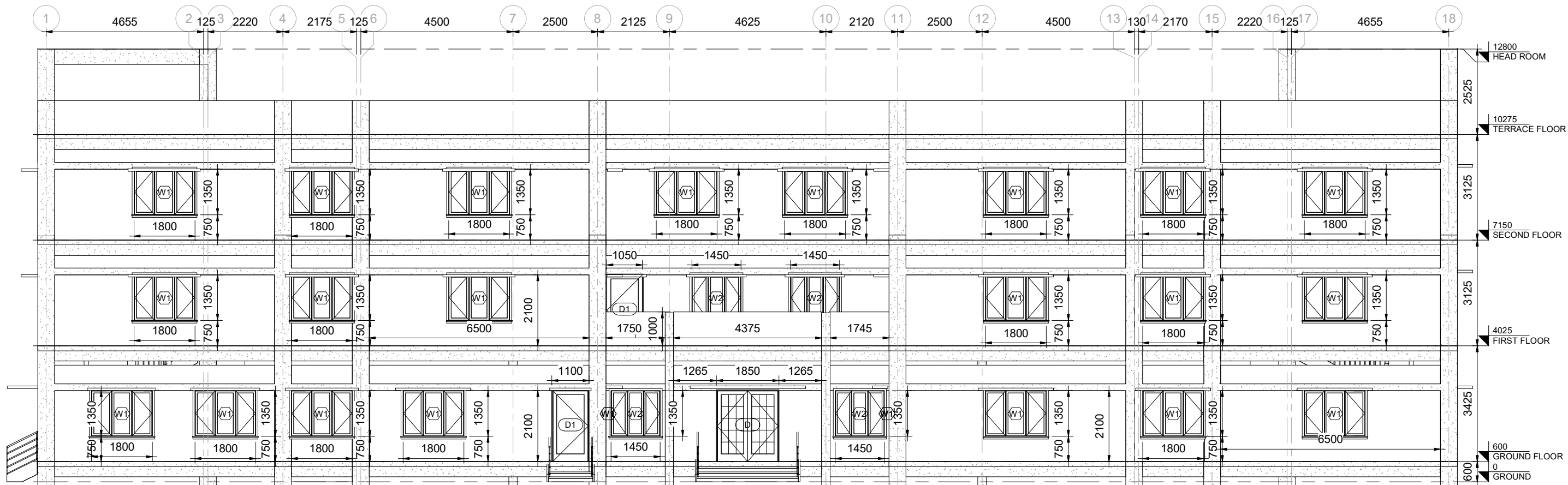
1 FRONT ELEVATION
