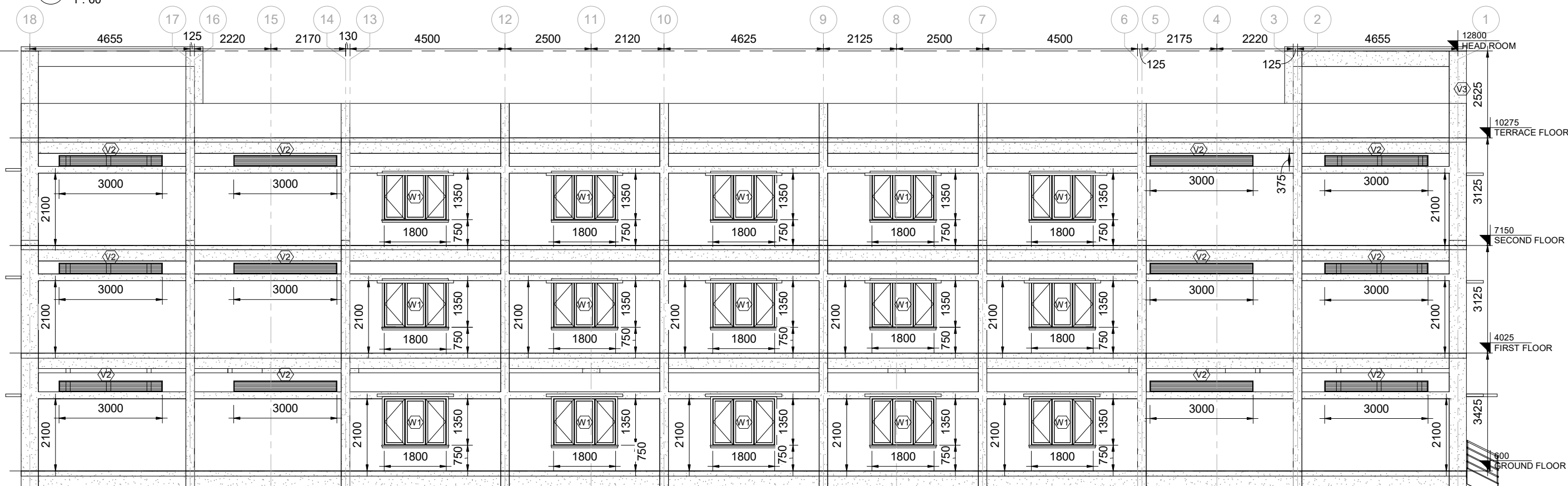
2 REAR ELEVATION
