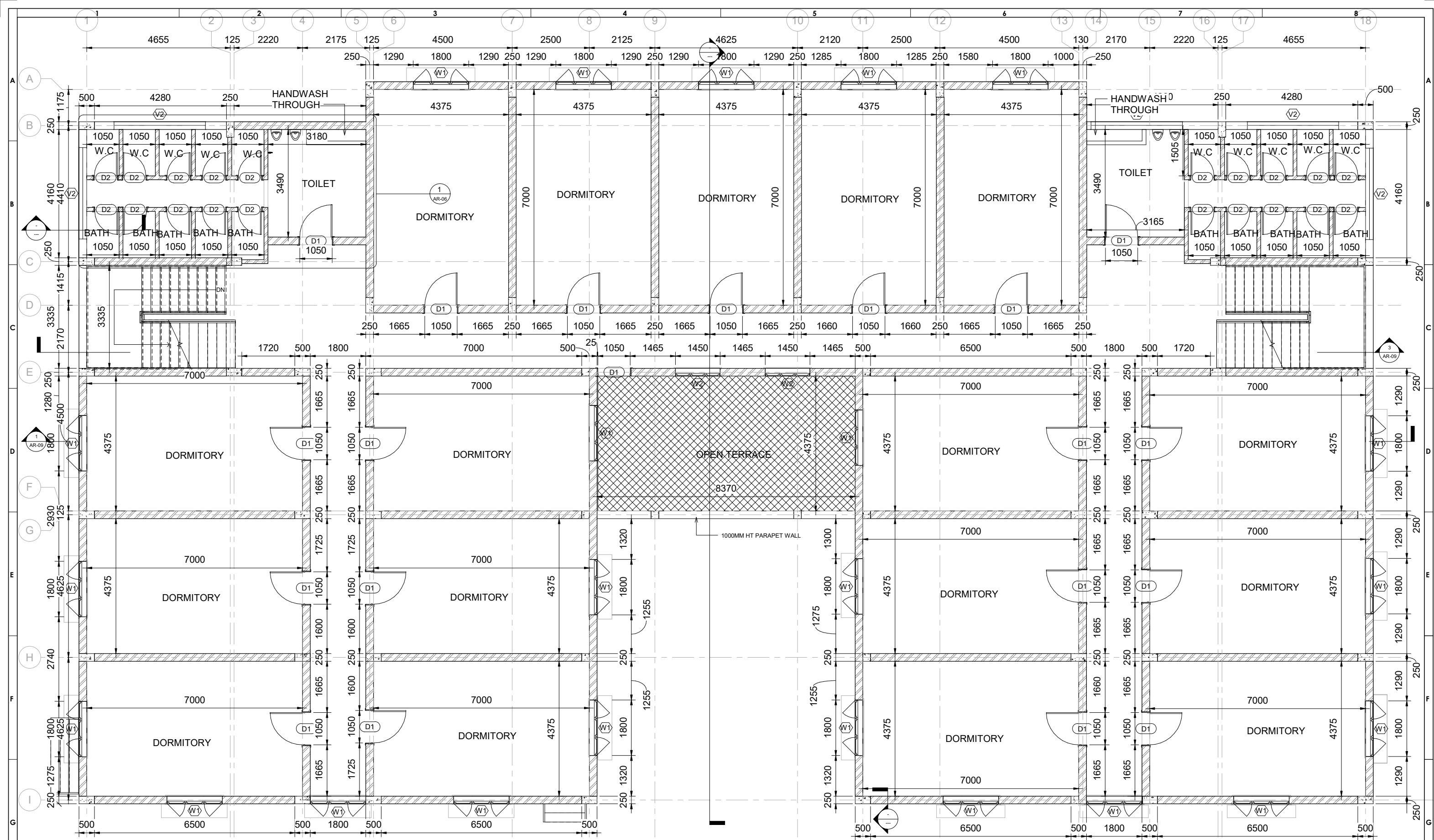
1 FIRST FLOOR PLAN 1 : 55
