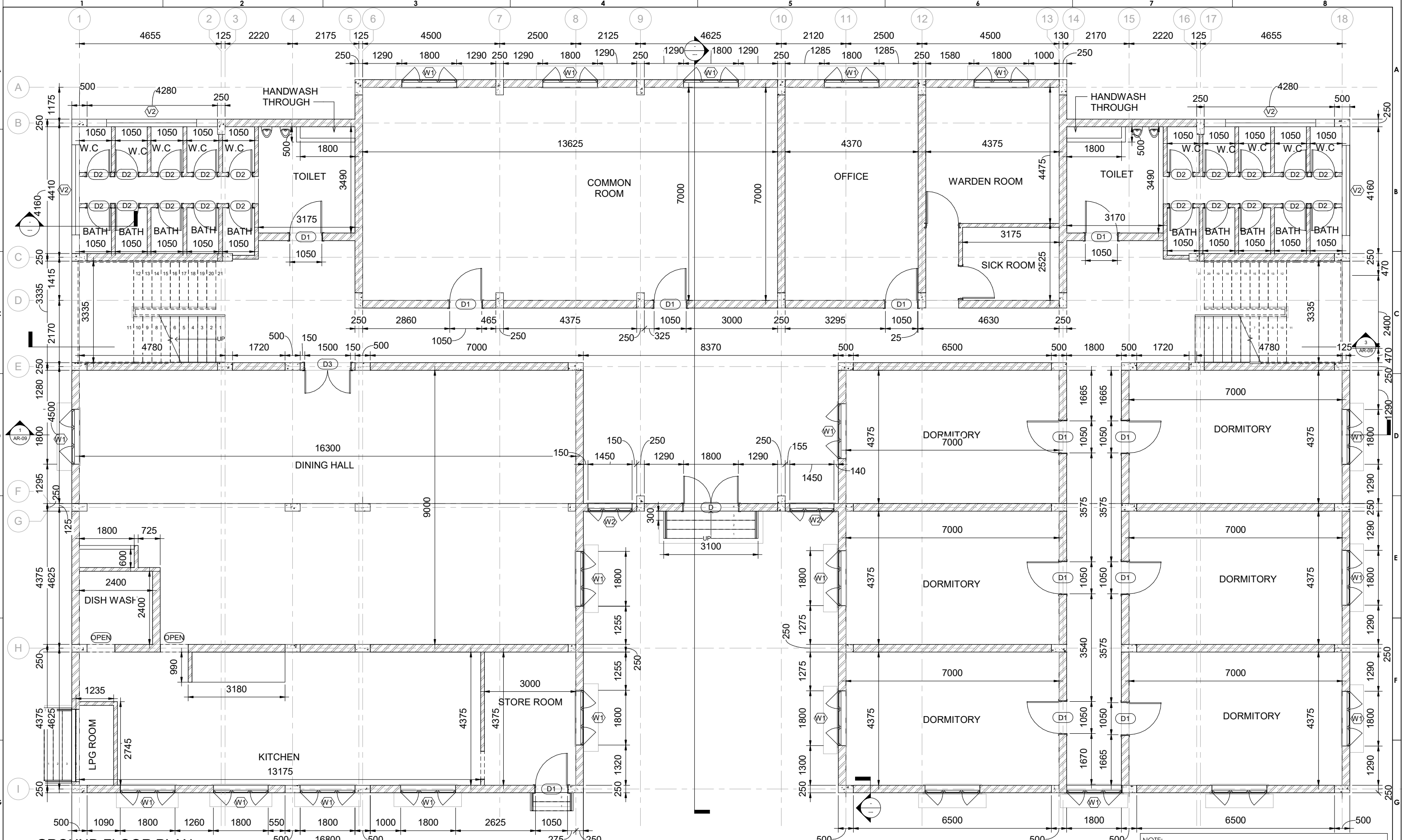
1 1 : 55 GROUND FLOOR PLAN
