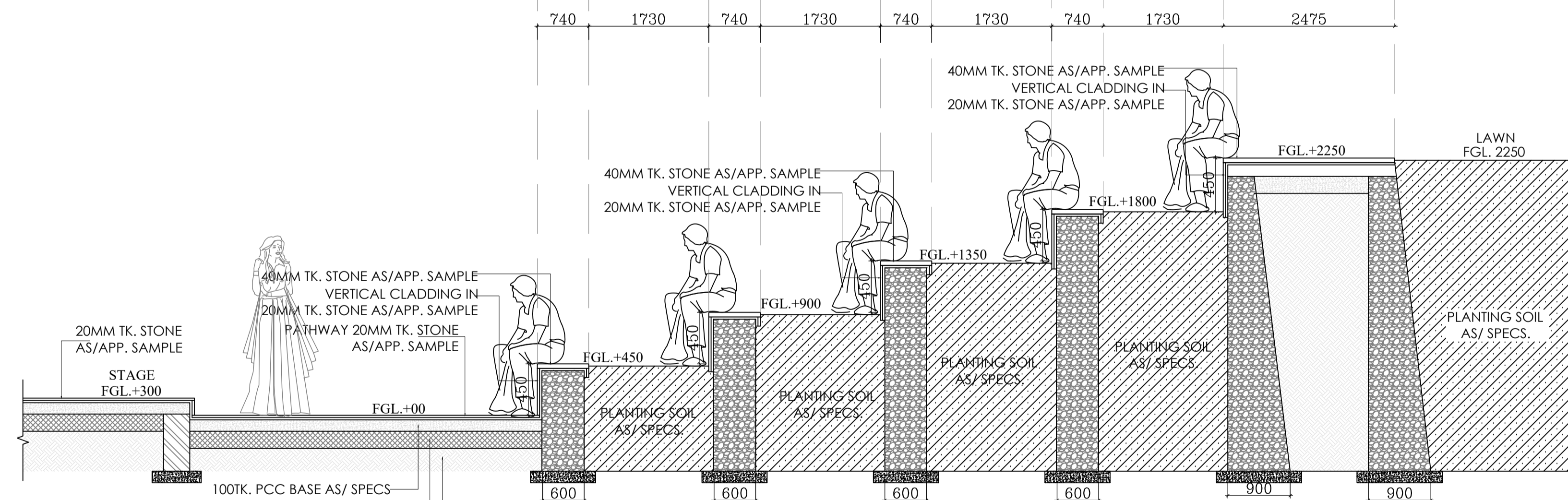
SECTION -A-A
