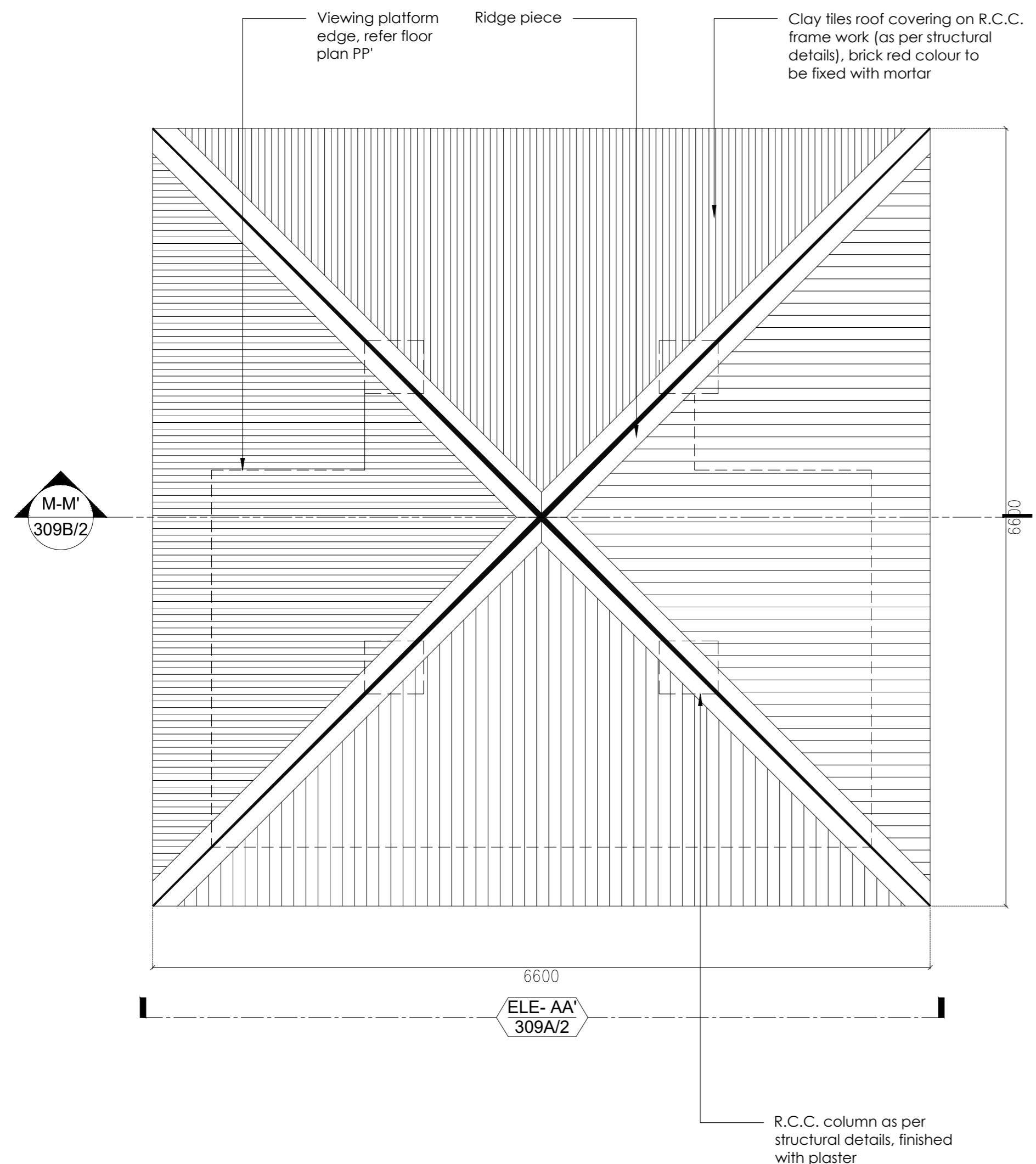
1 PLAN QQ' (Showing the roofing plan at LVL +13500 from N.G.L.)
