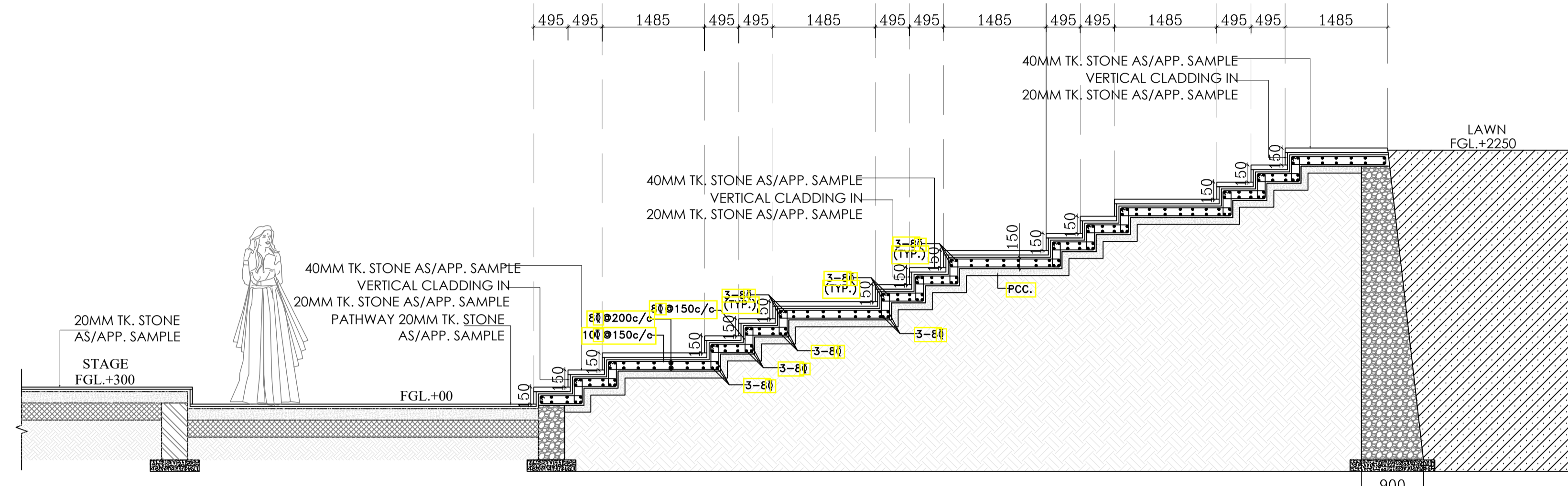
SECTION -B
