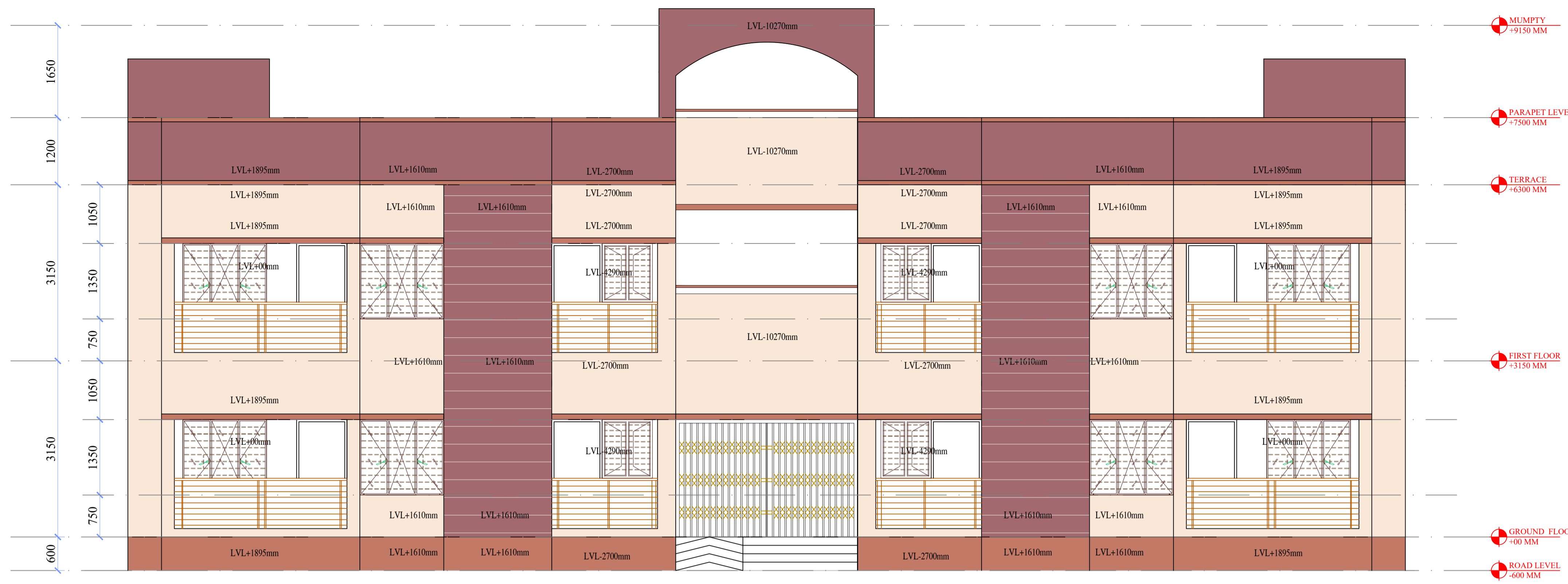
FRONT ELVATION
