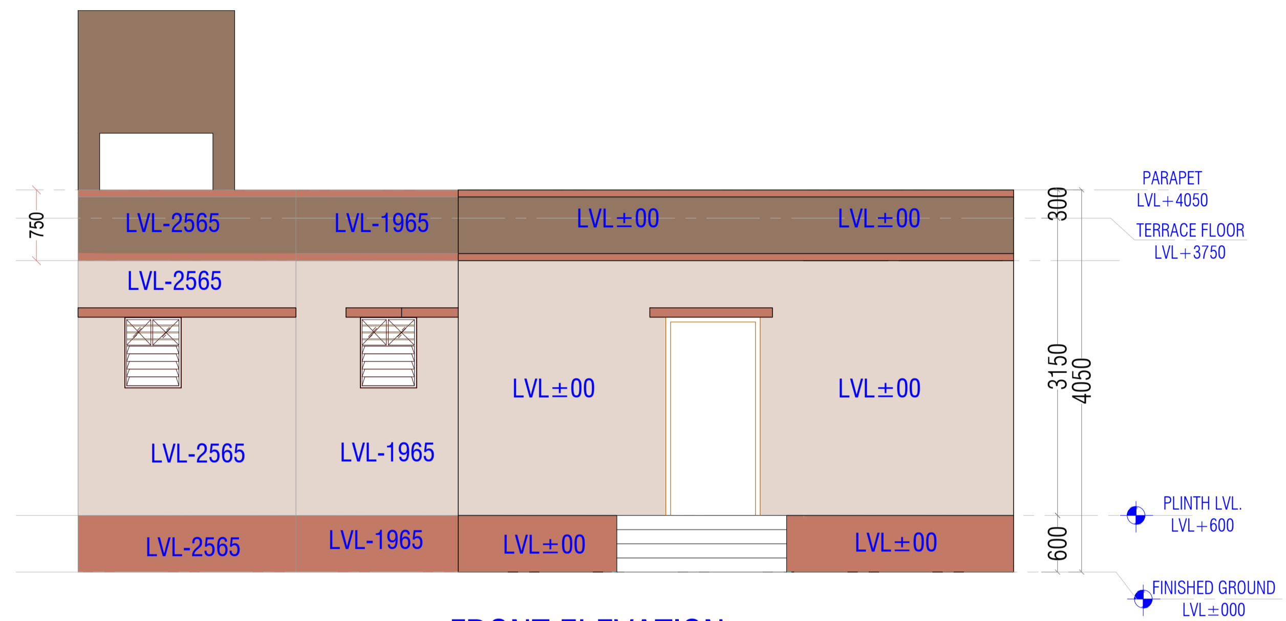
FRONT ELEVATION
