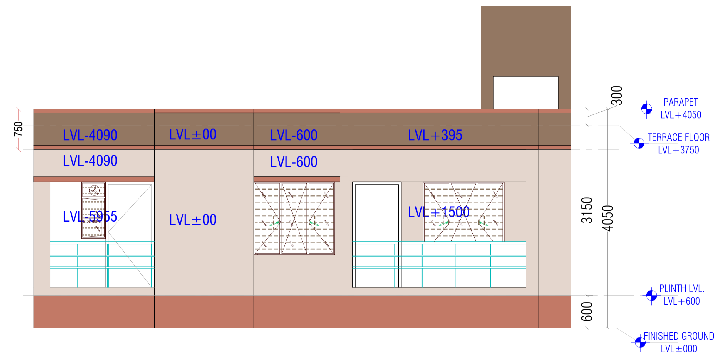
BACKSIDE ELEVATION
