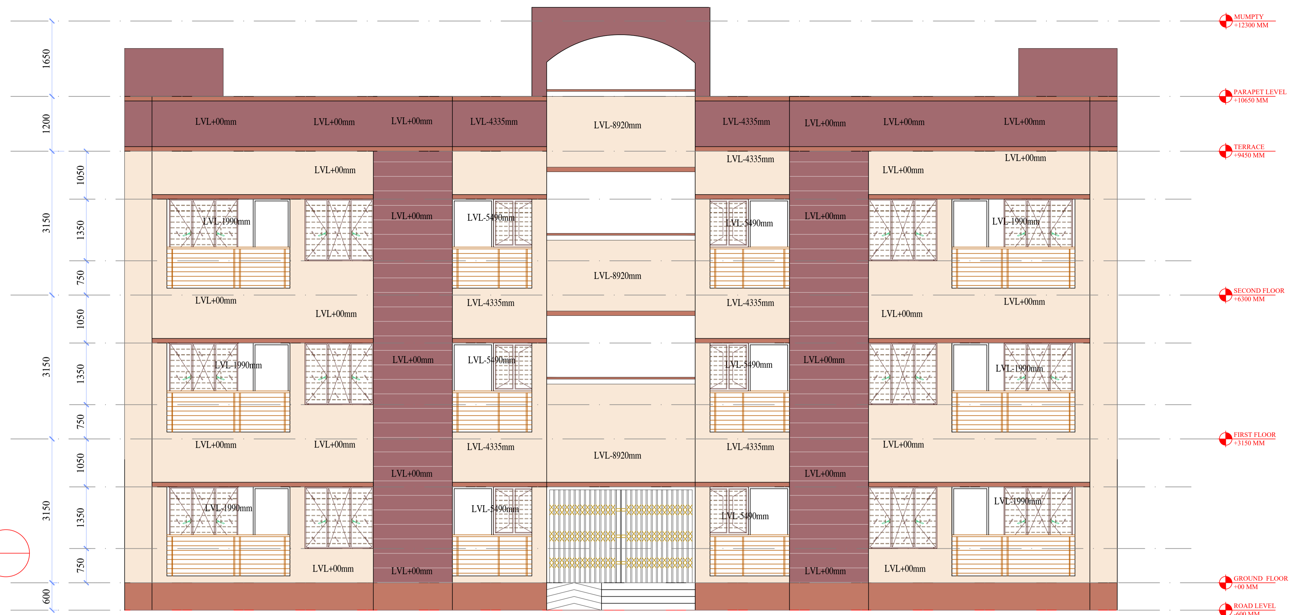
FRONT ELVATION
