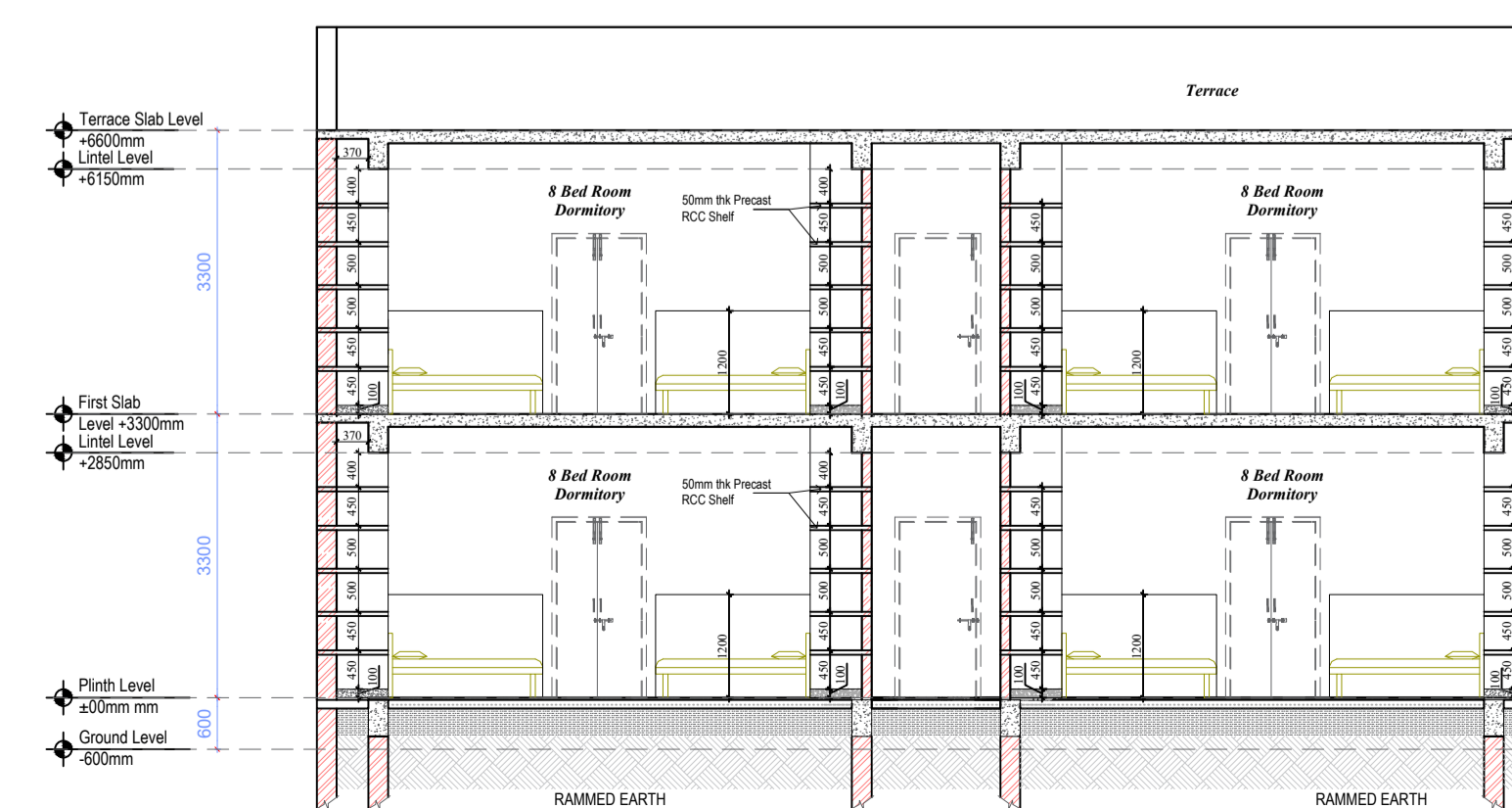
SECTION B-B
