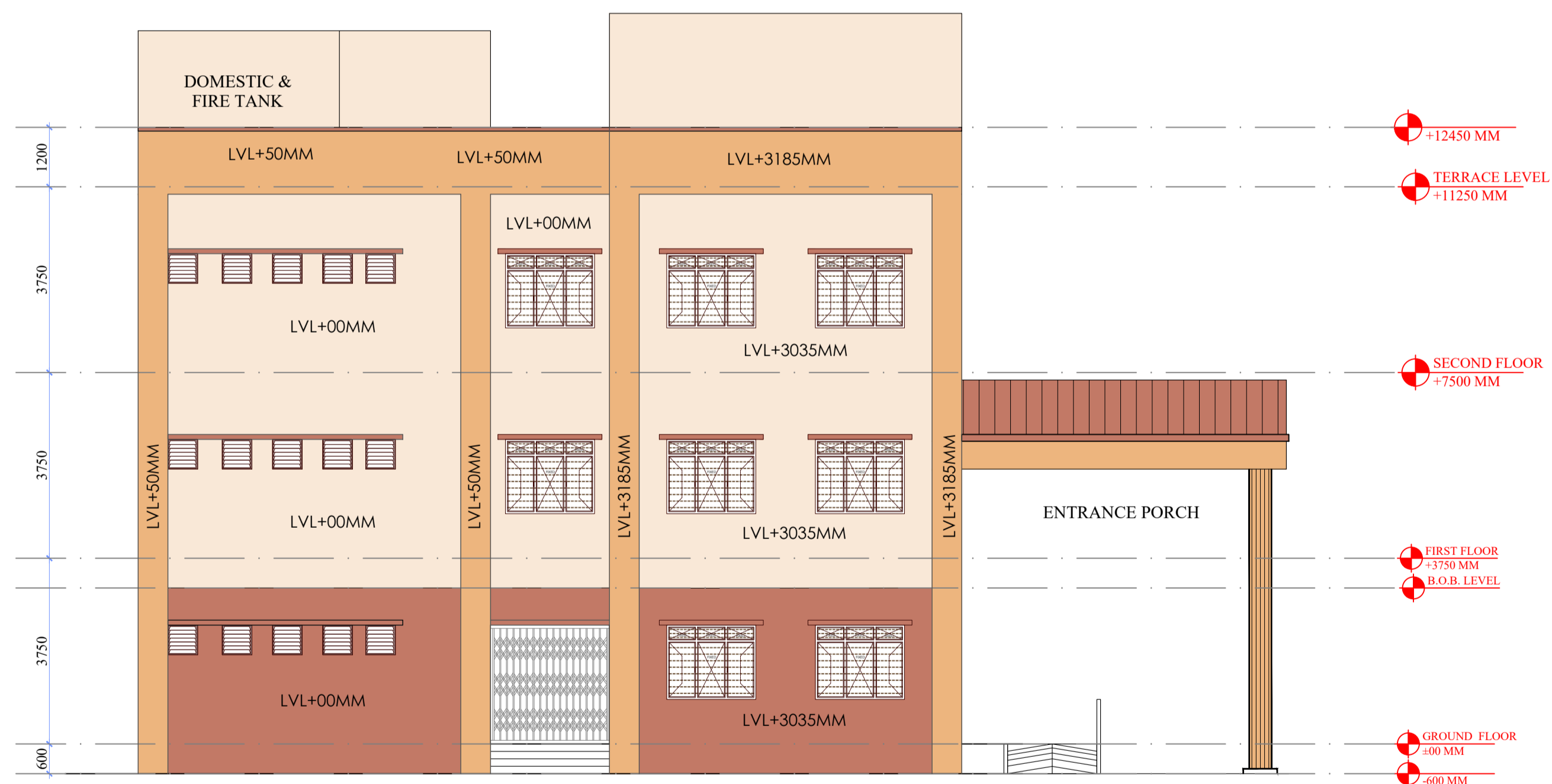
SIDE ELEVATION
