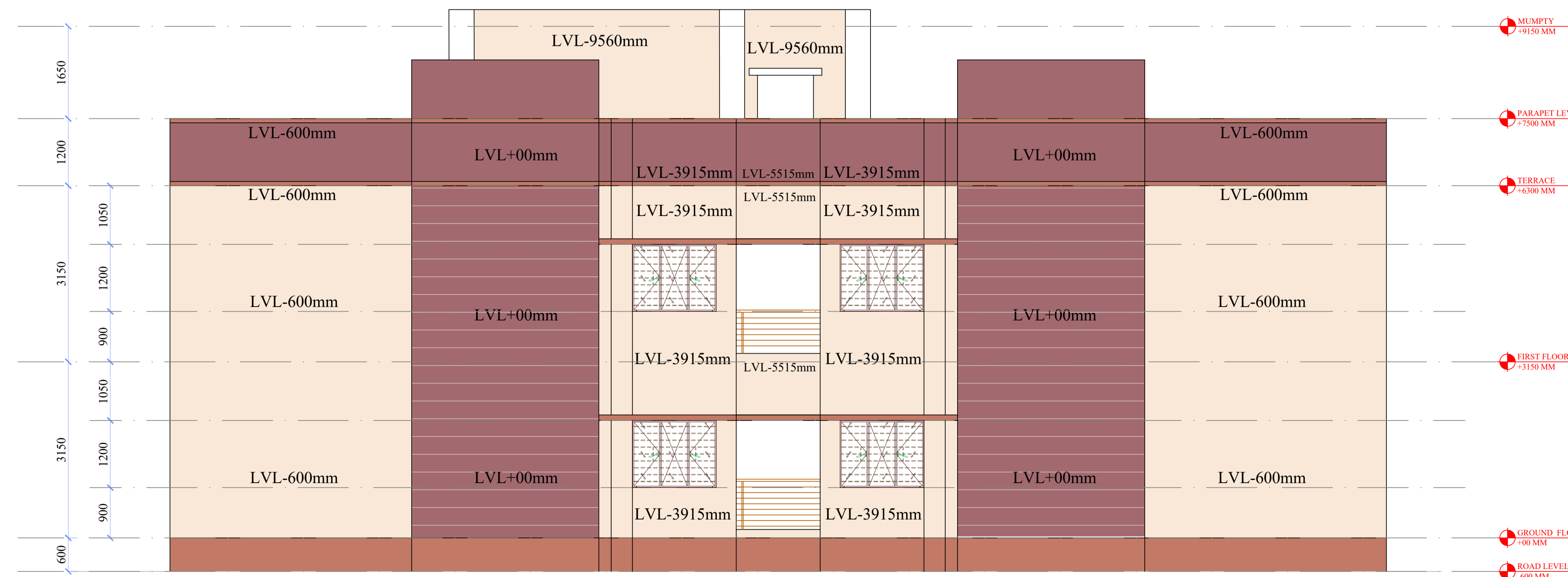
SIDE ELVATION
