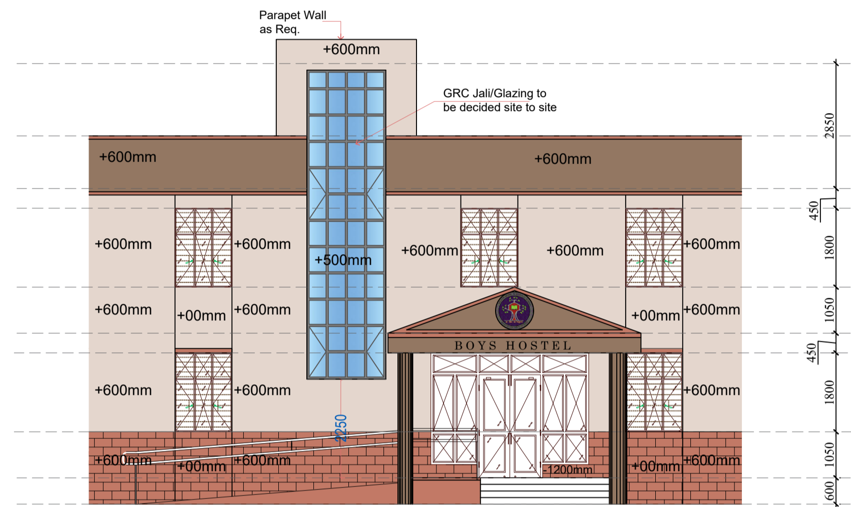
FRONT ELEVATION
