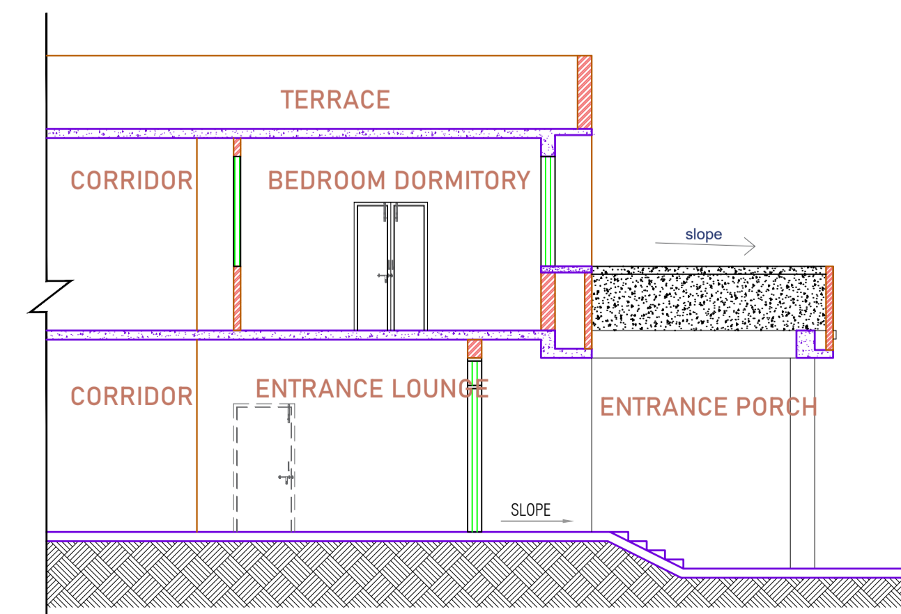
SECTIONAL VIEW A-A
