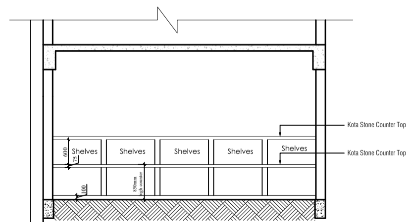
LAB RCC850MM HIGH COUNTER WITH SHELF ABOVE- RCC SHELVES DETAIL
