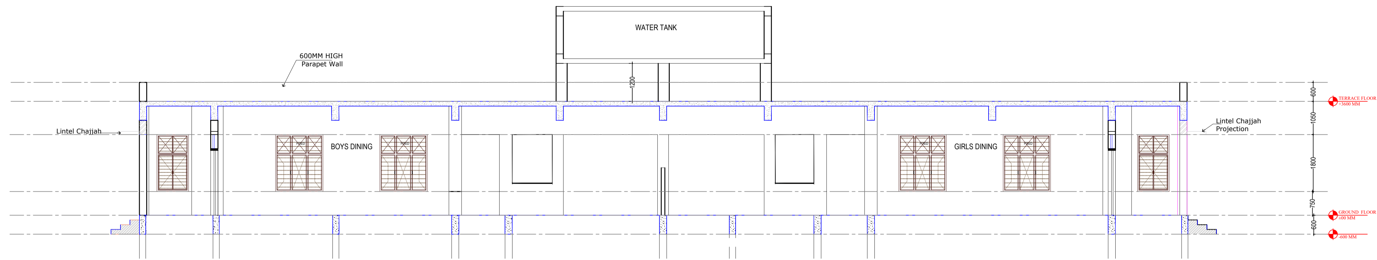
SECTION - AA
