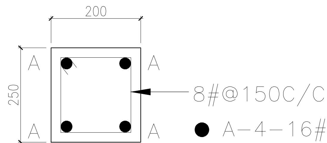
DETAIL OF C1
