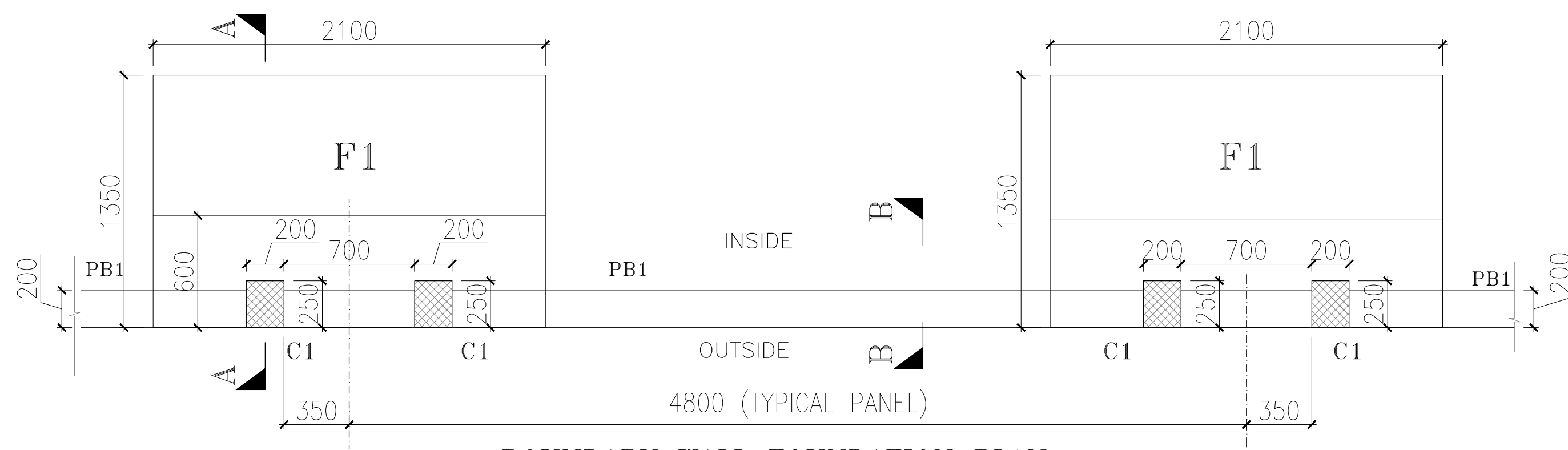
BOUNDARY WALL FOUNDATION PLAN
