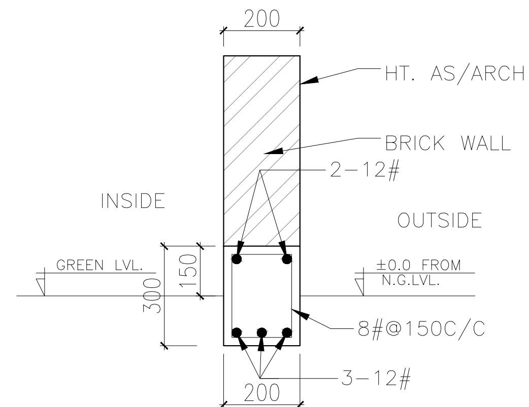
TYP. SEC.B-B BRICK WALL
