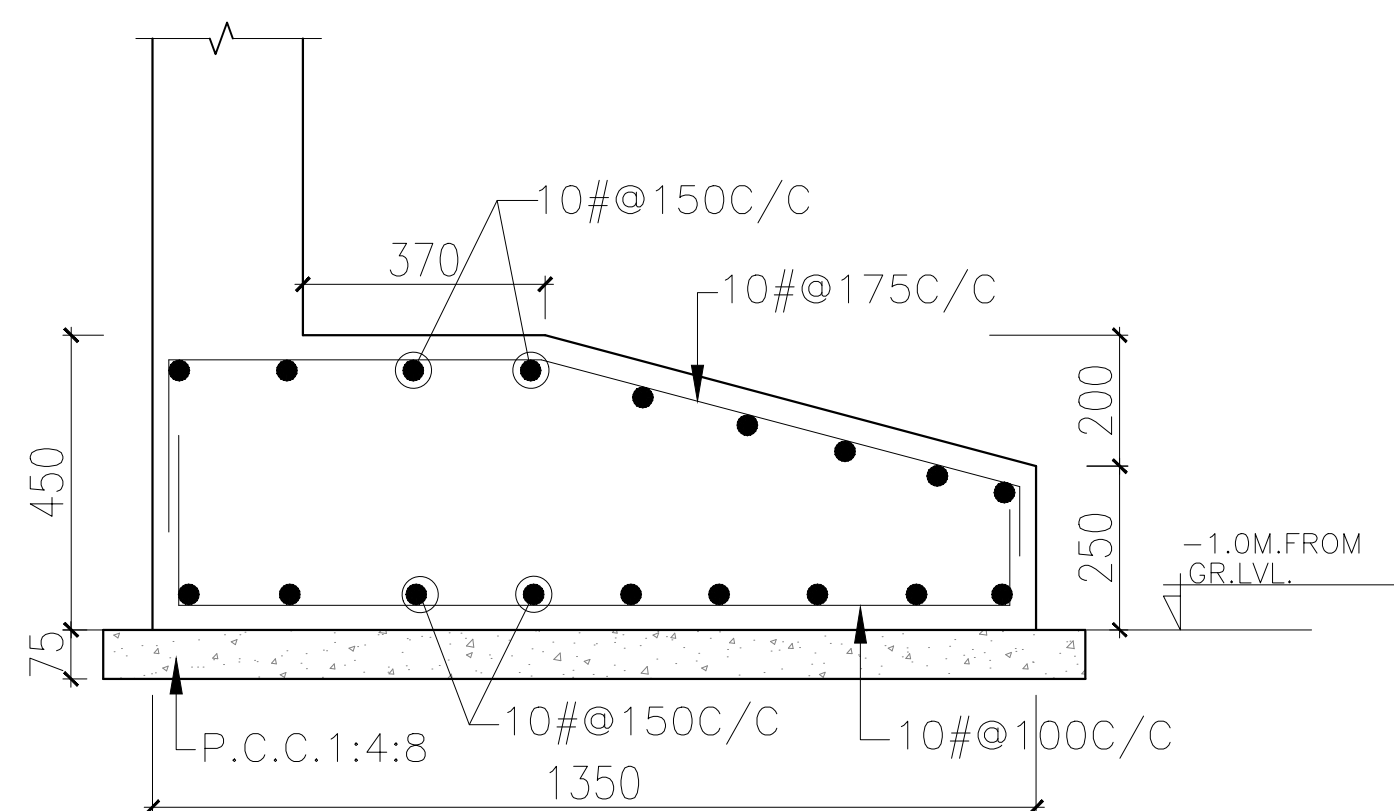
FOOTING SEC. A-A(F1)
