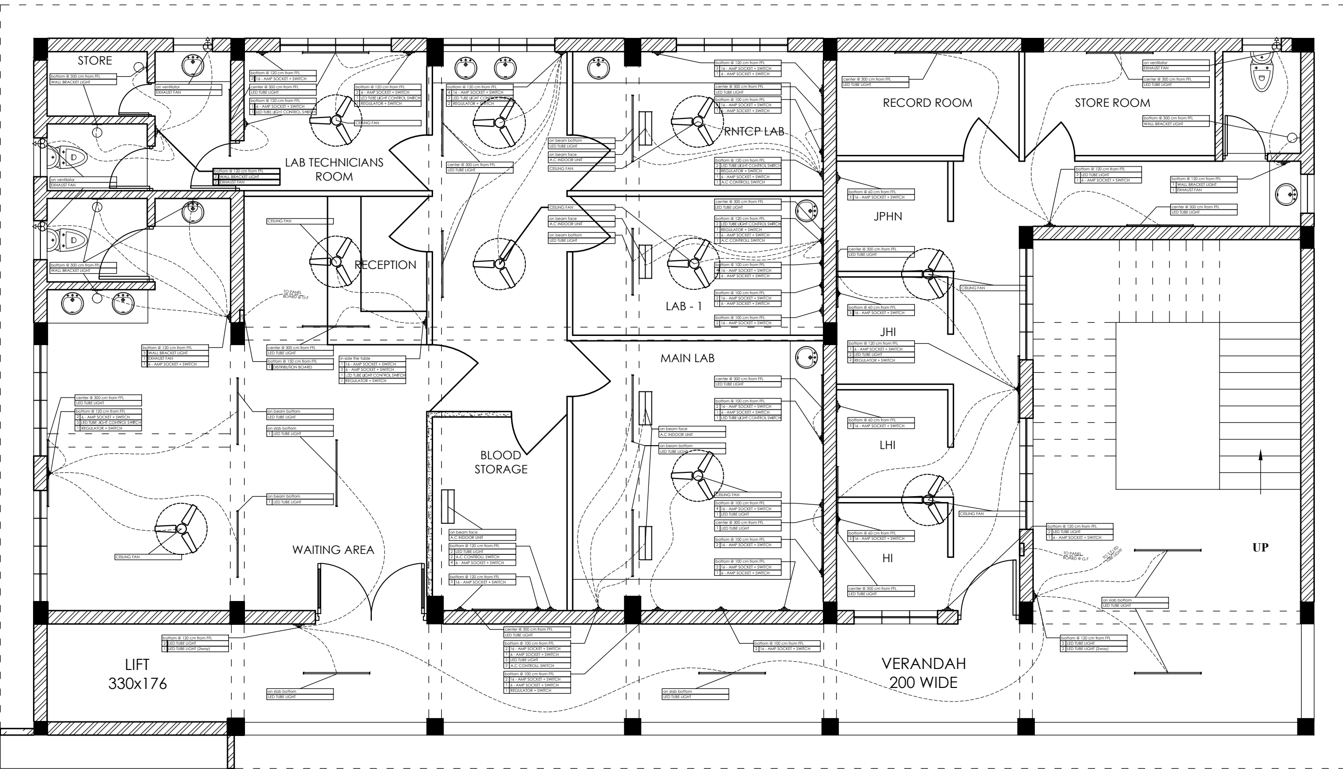
First Floor Plumbing and Electrical Drawing
