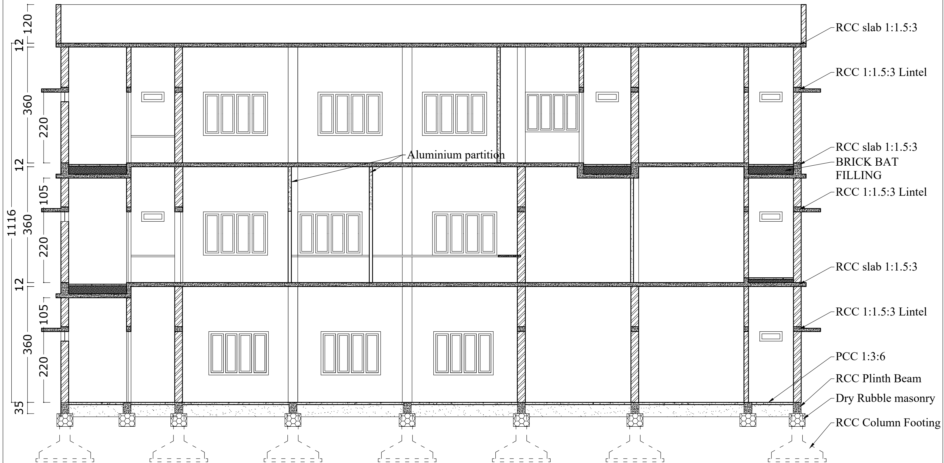
SECTION B-B
